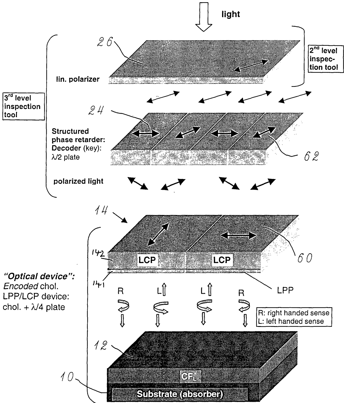
Fig. 4: 3 rd level LPP/LCP Security Device: Cholesteric type
