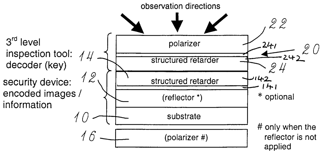
Fig. 2a: 3 rd level inspection mode
