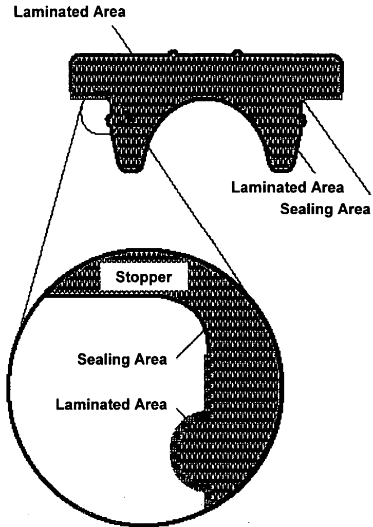
Figure 1: Sealing Area of Flurotec™ Closure
