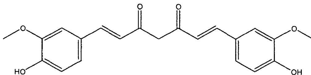
(1E,6E)-1,7-bis(4-hydroxy-3-methoxyphenyl)-6-heptadiene-3,5-dione (Curcumin)
