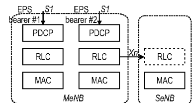
Fig. 22i Alternative 3D
