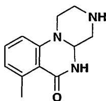
7-Methyl-1,2,3,4,4a,5-hexahydropyrazino[1,2-a]quinazolin-6-one
