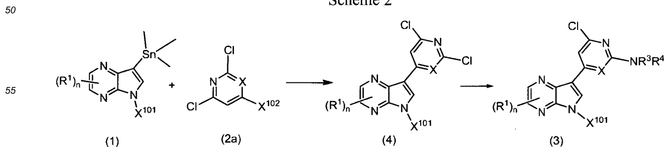
Scheme 2
