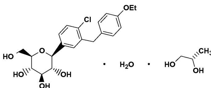
Compound 1a
