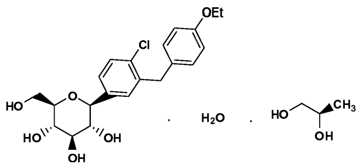
Ib (SD-3)
