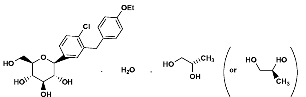
Compound Ia
