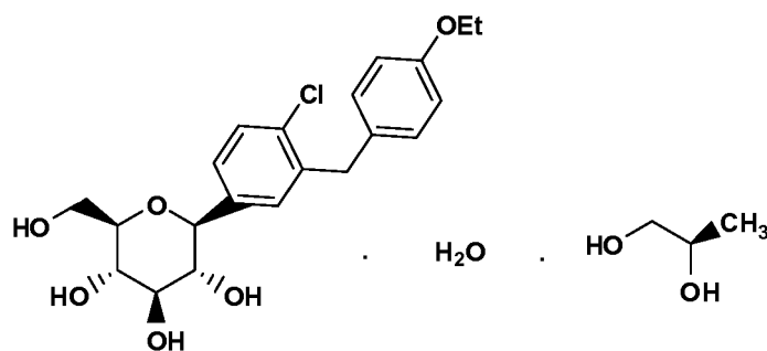
Compound Ib (SD-3)
