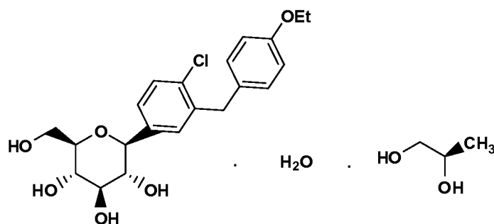
Compound Ib
