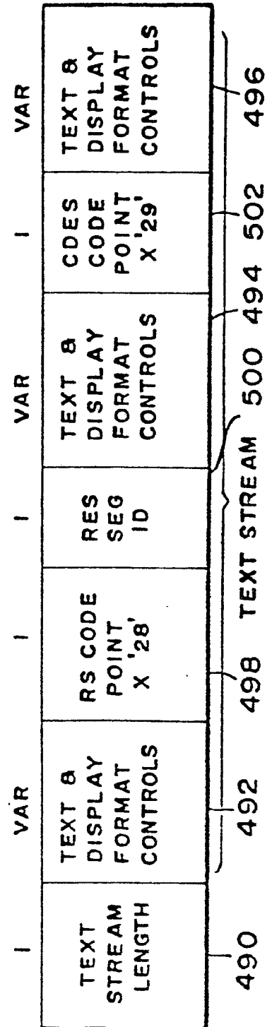
PAGE DESCRIPTION FIELDS OF INTERACTIVE DISPLAY MESSAGE
