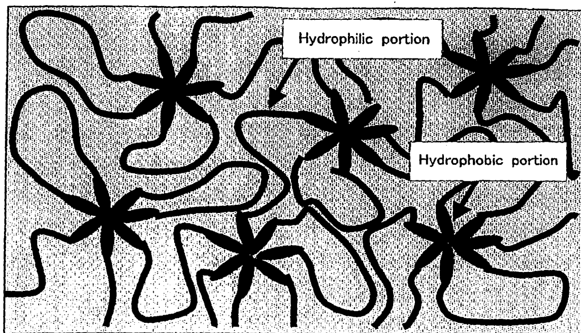
Copolymer(Associative thickener)
