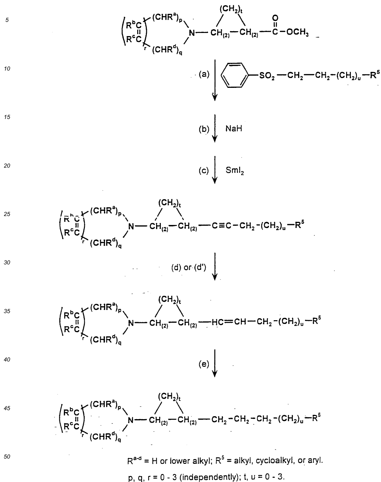
SCHEME 14:
