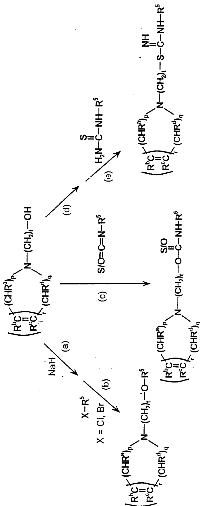
SCHEME 8:
