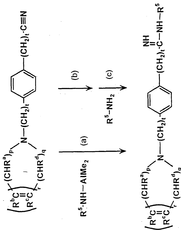
SCHEME 11:
