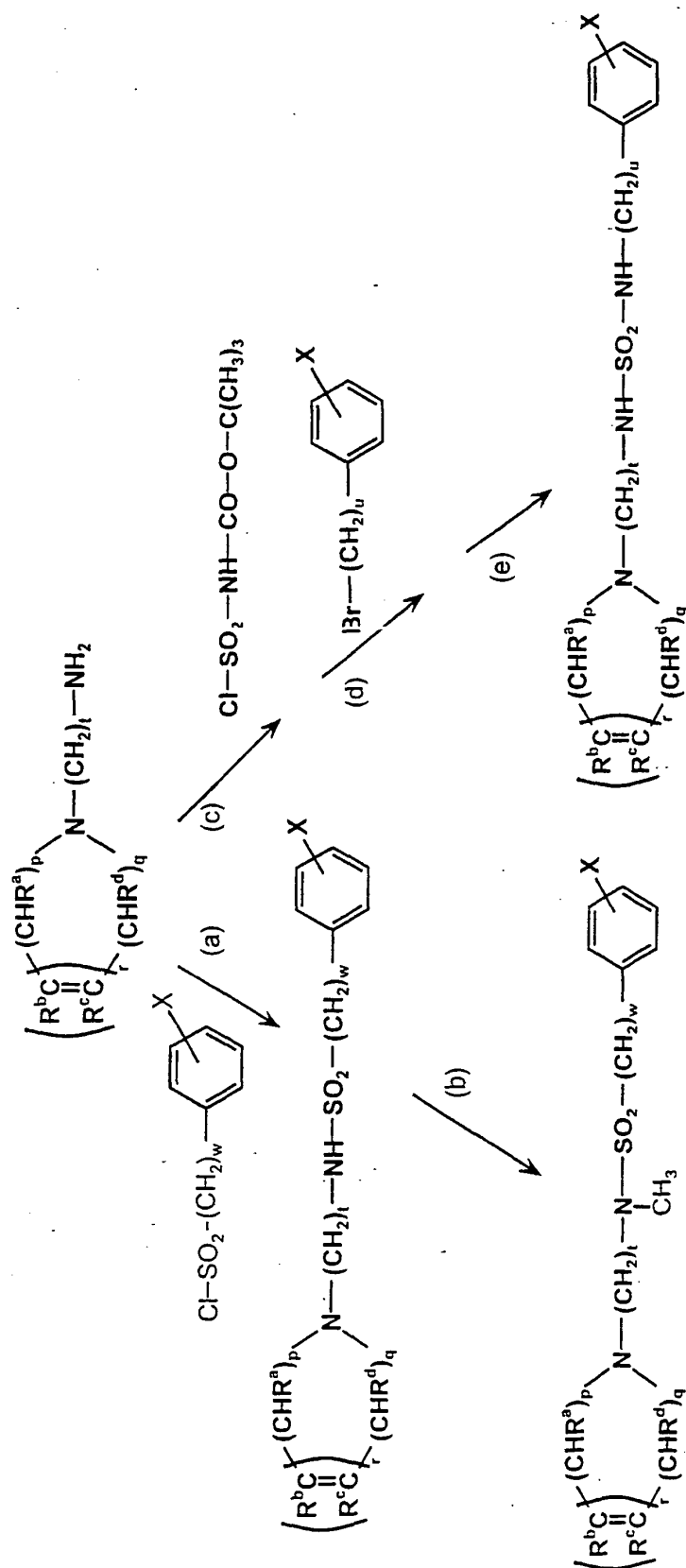
SCHEME 12
