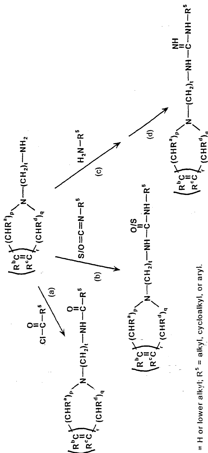
SCHEME 7:
