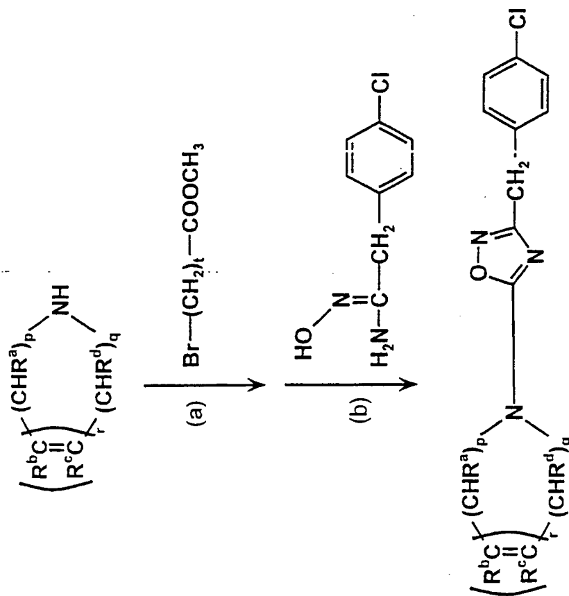
SCHEME 10:
