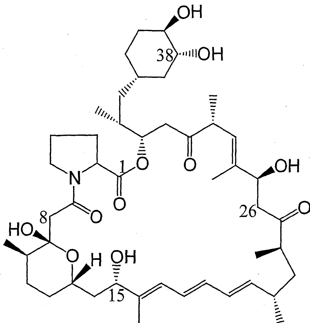
8-deoxy-15-O-desmethyl-26-desmethoxy-38-O-desmethyl polyrapamycin
