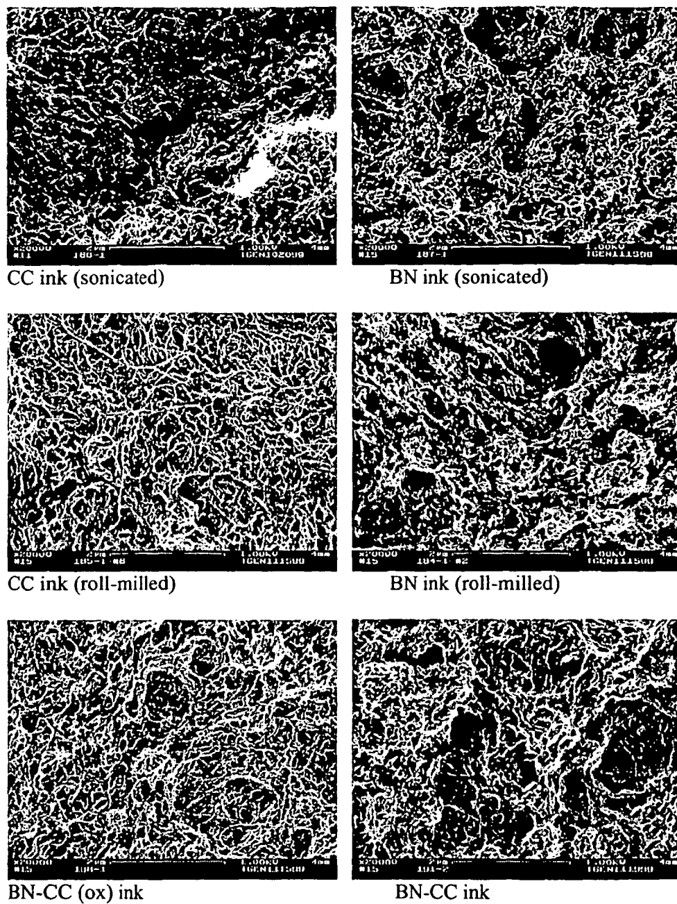
Figure 7 SEM images of fibril ink coating surface morphologies.
