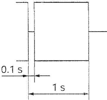
FIG. 5B BINARY 0 SIGNAL
