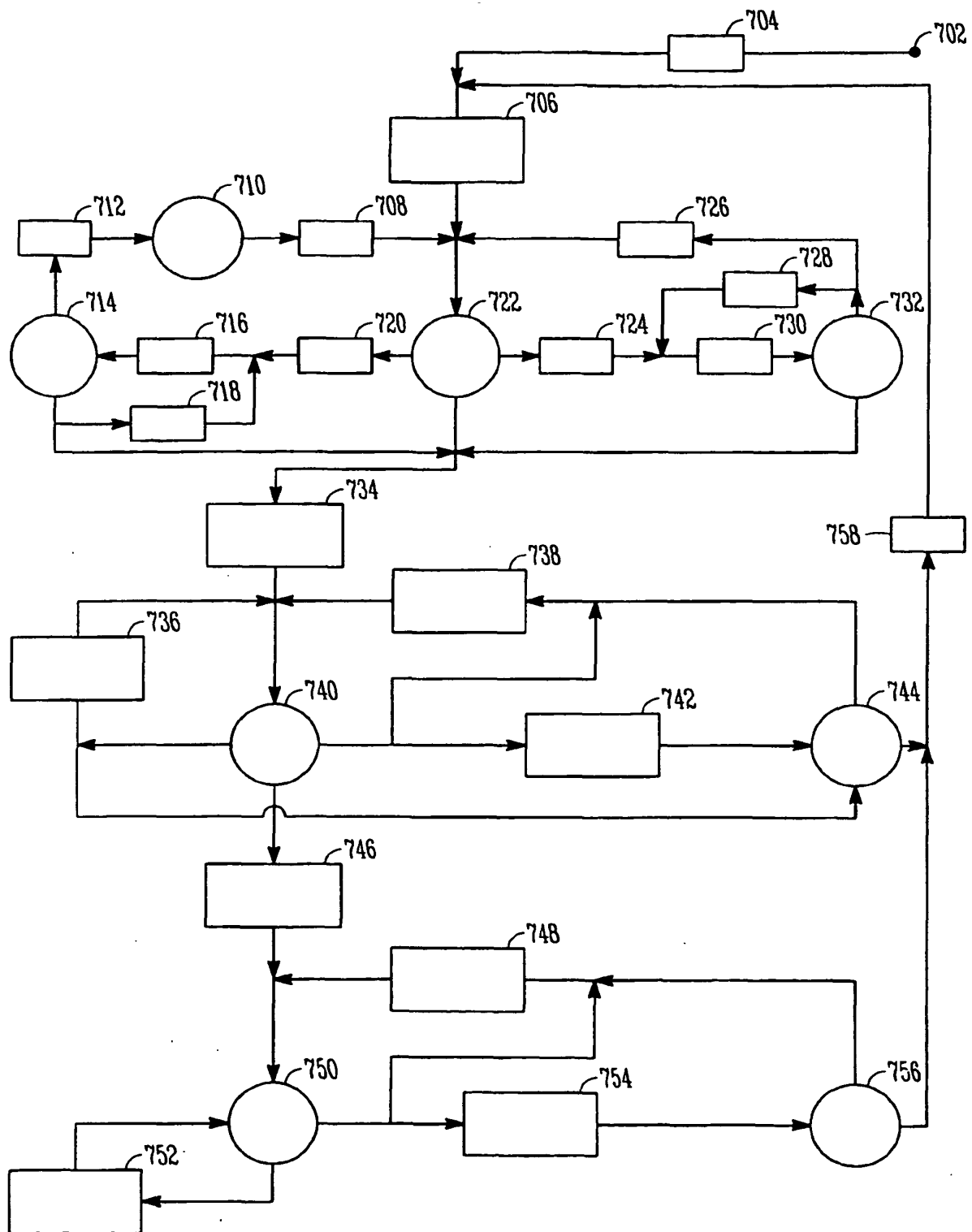
HOP ON ERROR FREQUENCY HOPPING STATE DIAGRAM PRM SIDE
