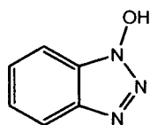
1-hydroxybenzotriazole
