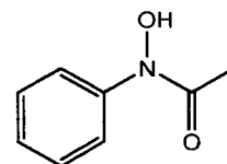
N-hydroxyacetanilide
