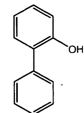
2-hydroxybiphenyl
