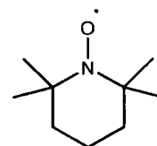
2,2,6,6-tetramethyl-1-piperidinyloxy (TEMPO)
