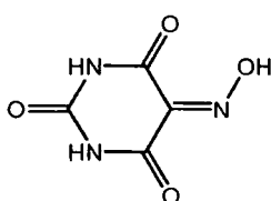
violuric acid
