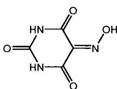
violuric acid
