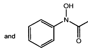
N-hydroxyacetanilide
