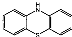
10-H-phenothazine
