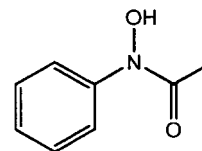
N-hydroxyacetanilide
