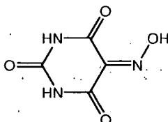
violuric acid
