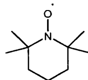
2,2,6,6-tetramethyl-1-piperadinyloxy (TEMPO)
