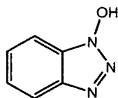
1-hydroxybenzotriazole
