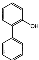
2-hydroxybiphenyl
