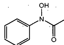
N-hydroxyacetanilide
