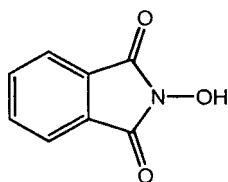
N-hydroxyphthalimide
