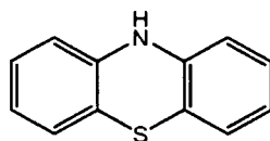
10-H-phenothazine
