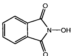
N-hydroxyphthalimide
