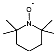
2,2,6,6-tetramethyl-1-piperadinyloxy (TEMPO)
