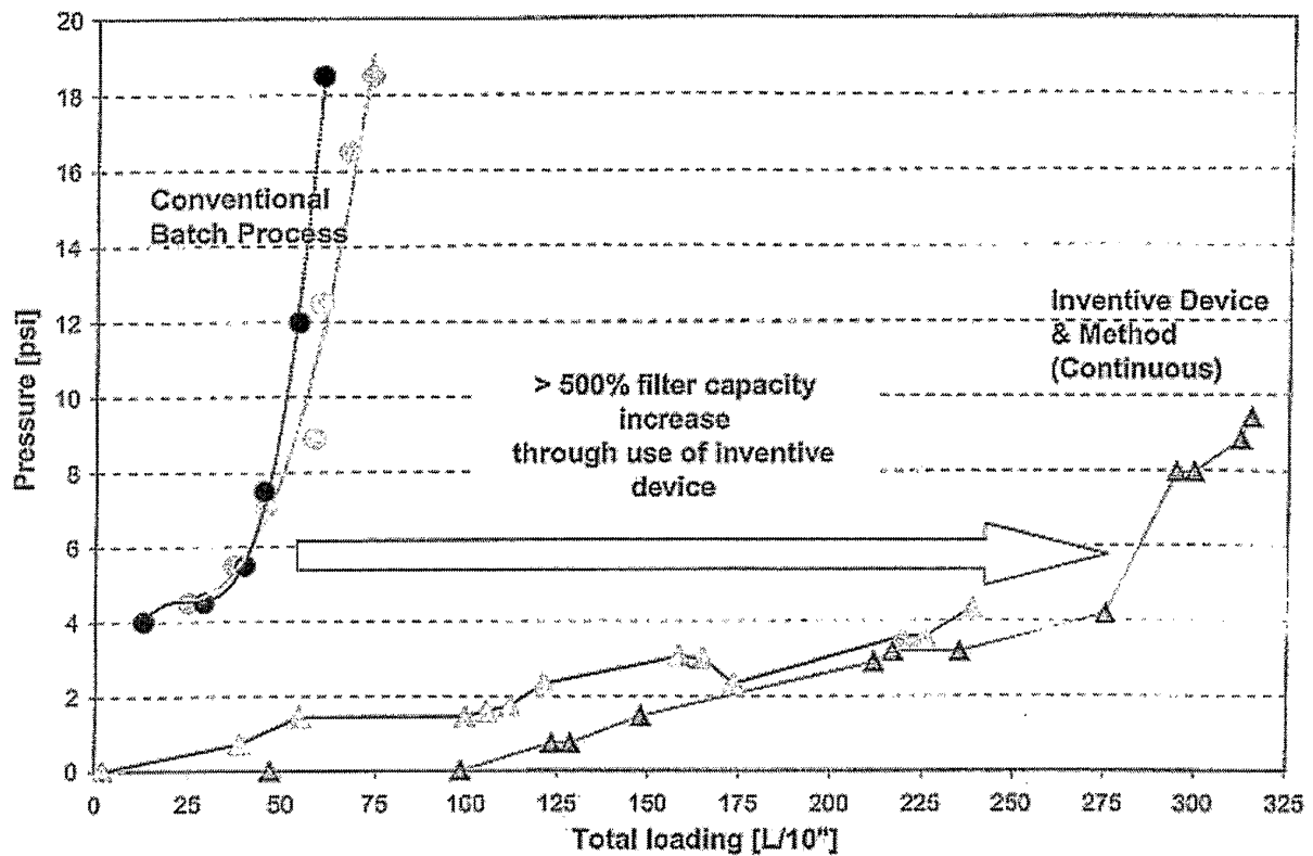
Figure 8: Example comparison of total load capacities per 10" of filter capsule for conventional batch process and embodiment of inventive device and method for continuous particle removal (integrated continuous filtration process) using identical commercial filter capsules. Example method producing recombinant blood coagulation Factor VIII shown.
