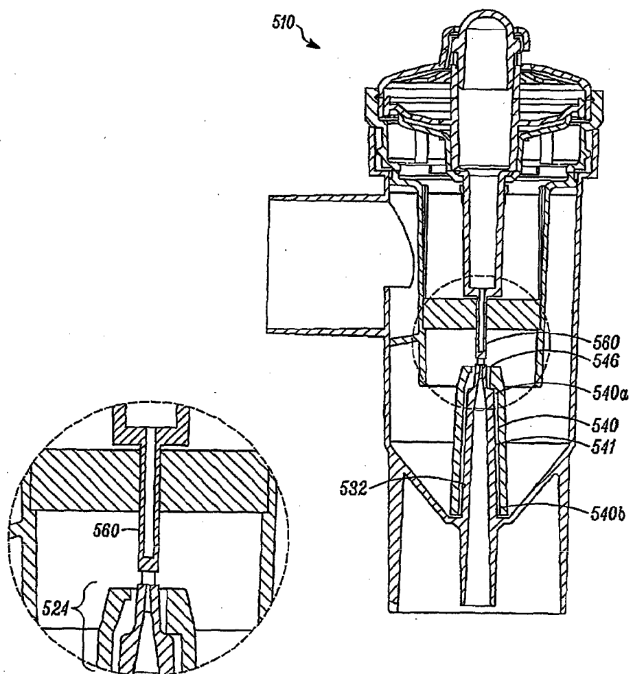
FIG. 9 Other Commercially Available Nebulizer - Modified Dimensions
