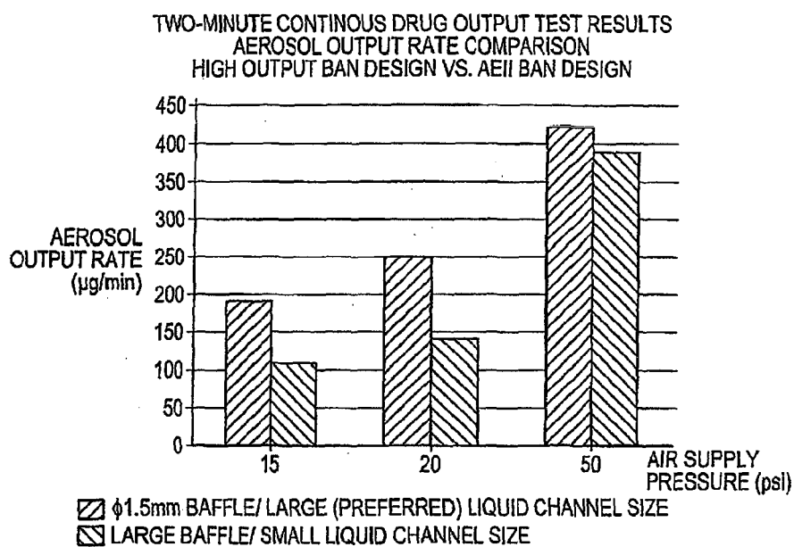
FIG. 10 Aerosol Output Rate, Modified AEII BAN vs AEII BAN
