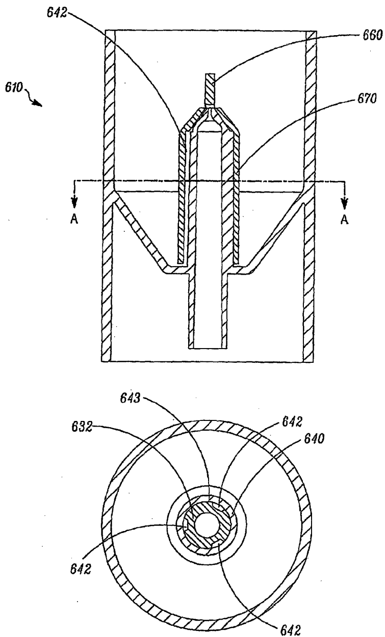
FIG. 15 Other Commercially Available Nebulizer - Baseline Device
