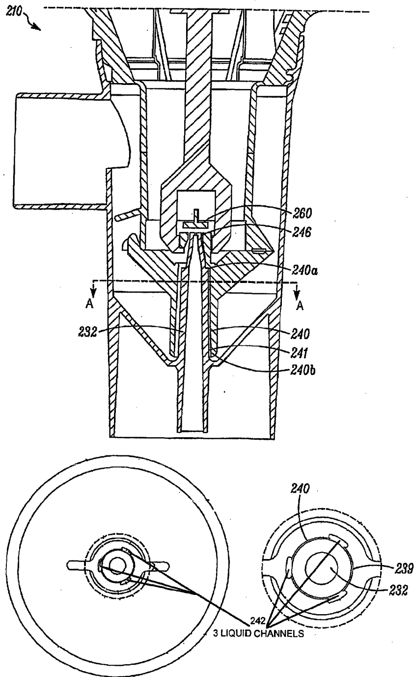
FIG. 4 AEII BAN - Baseline Device
