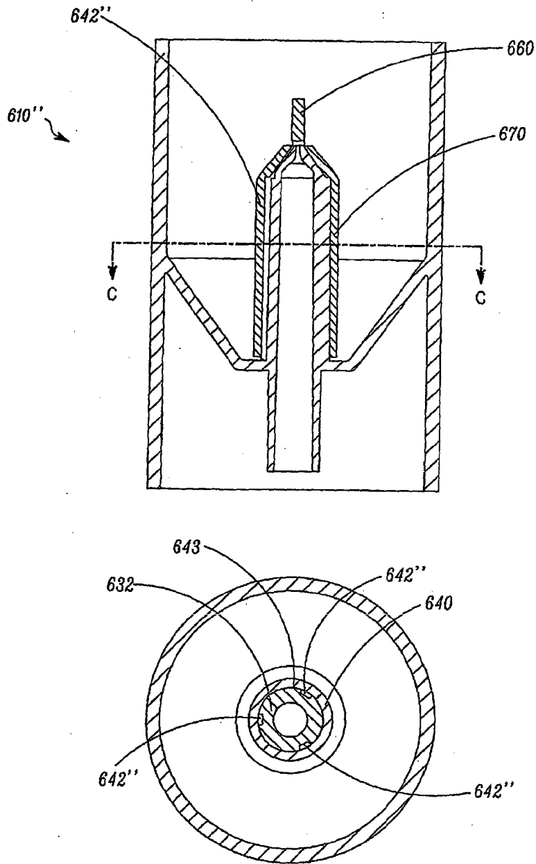
FIG. 17 Other Commercially Available Nebulizer - Liquid Channel Volume Increased by 60%
