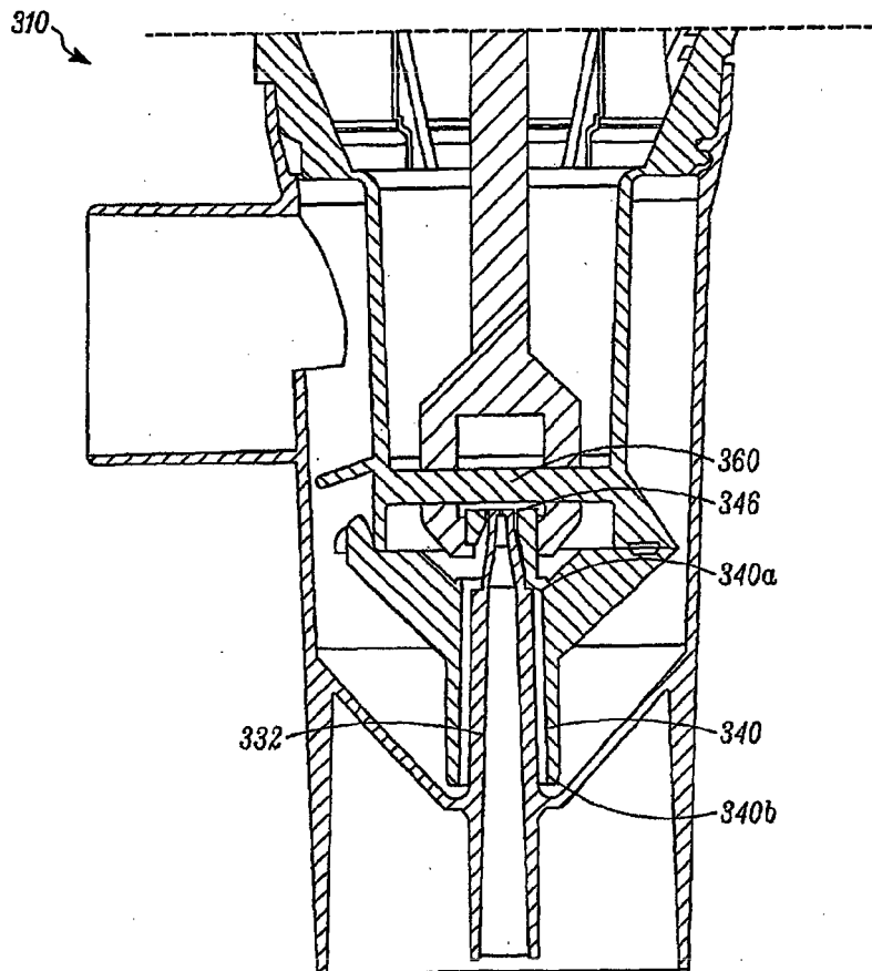
FIG. 7 AEII BAN with rib diverter - Alternative Dimensions
