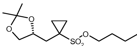
(R)-6 .
