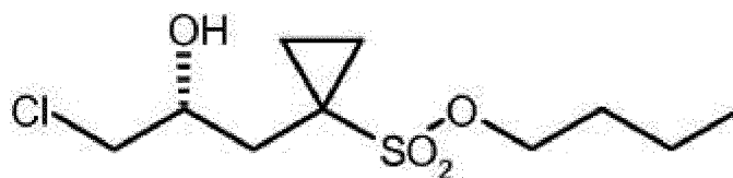
(R)-3;
