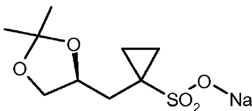
(S)-7
