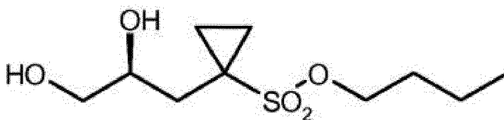
(S)-5
