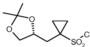
30 (R)-10
