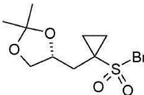
(R)-10-Br;
