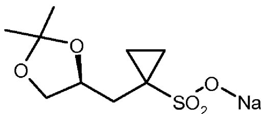
(S)-7
