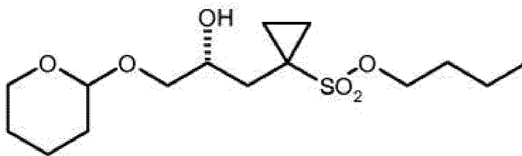
(R)-9b.
