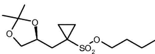
(S)-6
