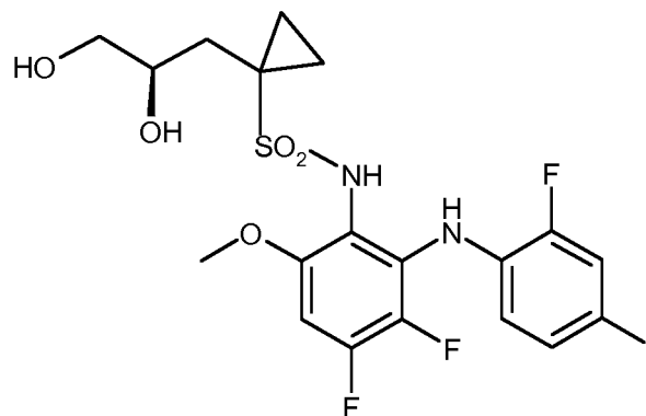
(R)-14,
