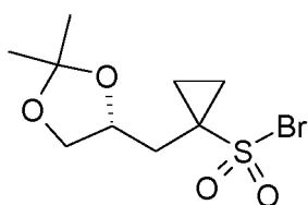
(R)-10-Br
