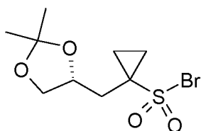
(R)-10-Br
