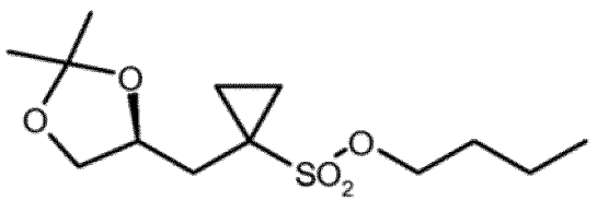
(S)-6 ;
