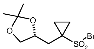
(R)-10-Br
