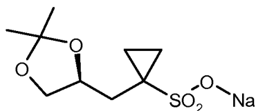
(S)-7
