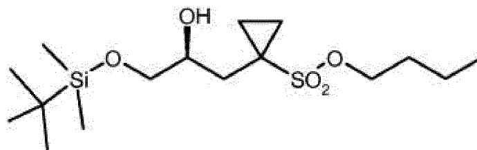
20 (S)-9a;
