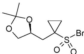
(S)-10-Br.
