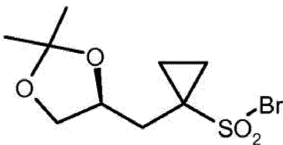
(S)-10-Br
