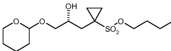
(R)-9b ;
