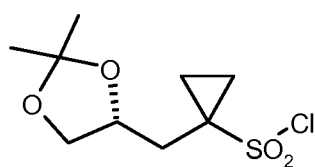
(R)-10
