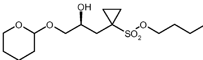
(S)-9b ;
