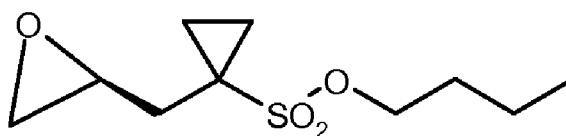
(S)-4
