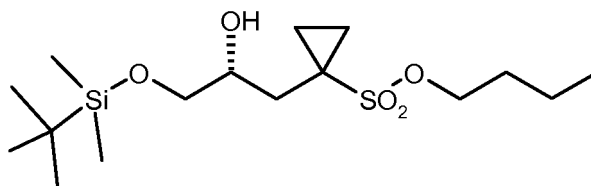
(R)-9a ;
