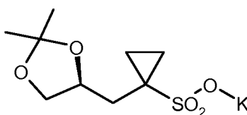
(S)-7' ;
