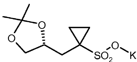
(R)-7' ;
