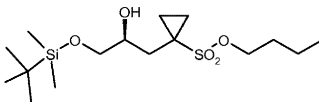
(S)-9a ;
