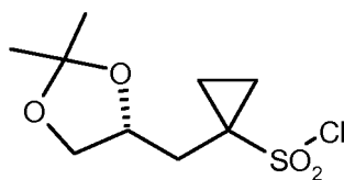
(R)-10
