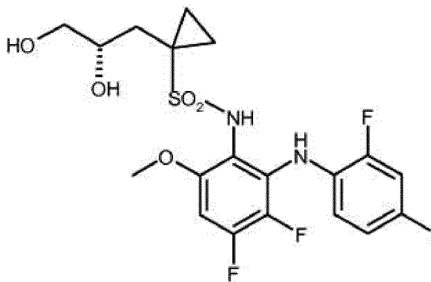
(S)-14.
