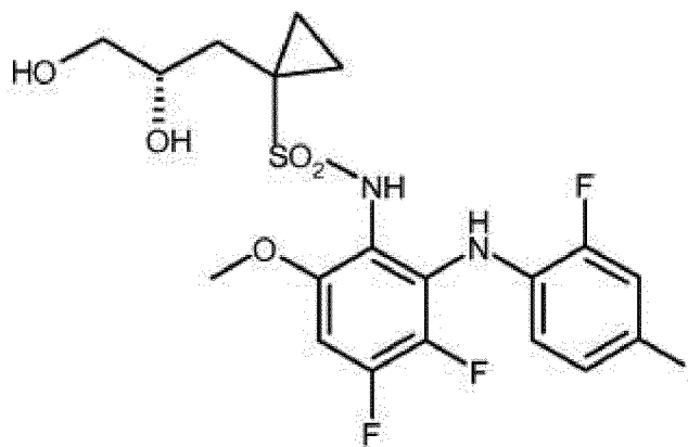
(S)-14;
