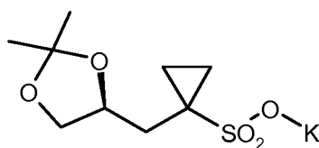
(S)-7'
