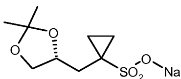
(R)-7
