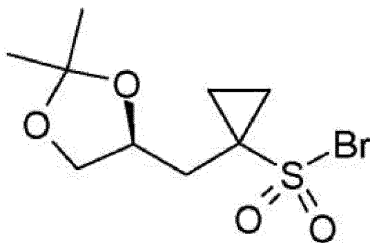
(S)-10-Br;
