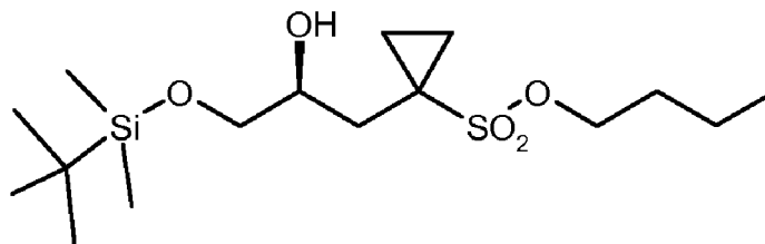
(S)-9a ;
