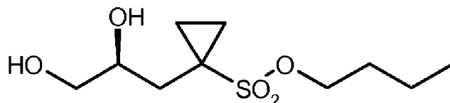
(S)-5
