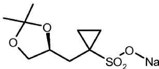
(S)-7
