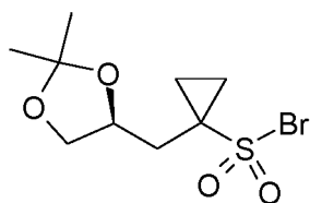
35 (S)-10-Br
