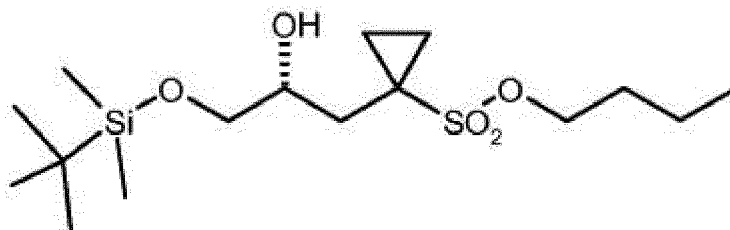
35 (R)-9a;
