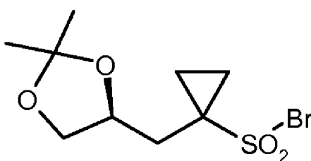
(S)-10-Br
