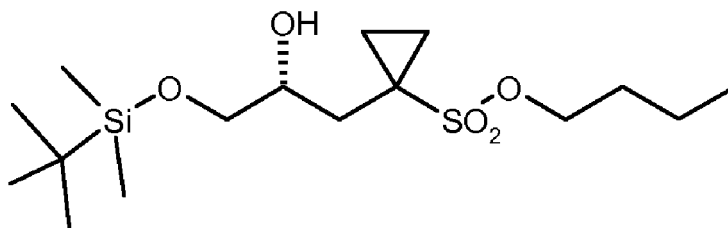
(R)-9a ;
