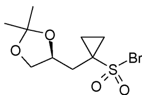
(S)-10-Br ;
