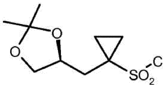
(S)-10;
