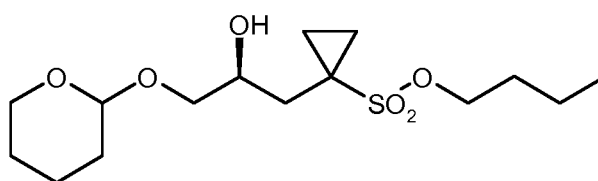
(S)-9b ;
