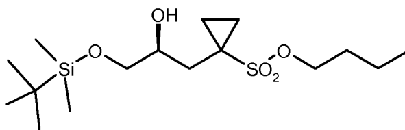
(S)-9a ;
