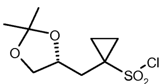
(R)-10
