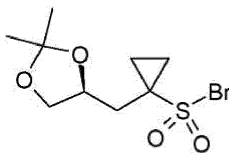
(S)-10-Br;
