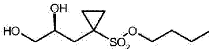
(S)-5;
