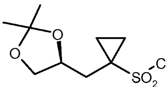
(S)-10
