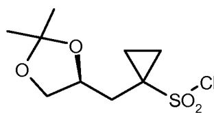
30 (S)-10
