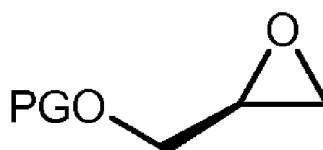
(S)-8,
