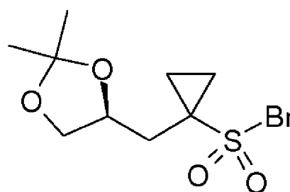
(S)-10-Br ;
