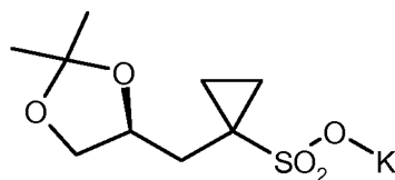
(S)-7'
