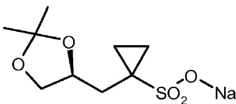
(S)-7
