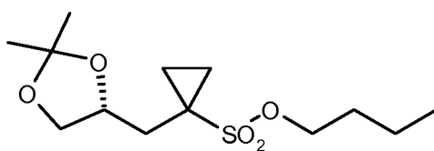
(R)-6
