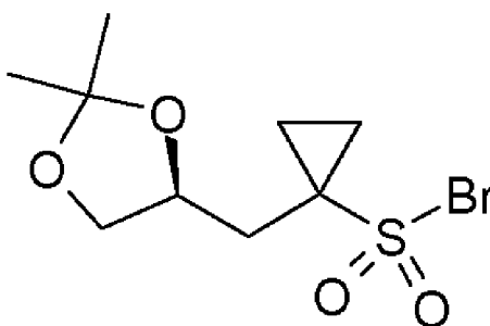
(S)-10-Br ;
