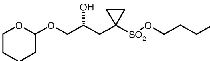
(R)-9b.
