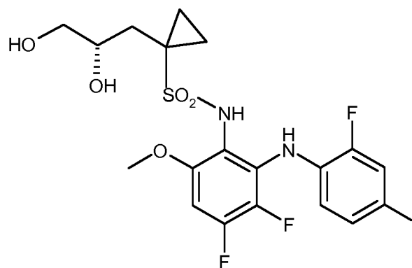
(S)-14,
