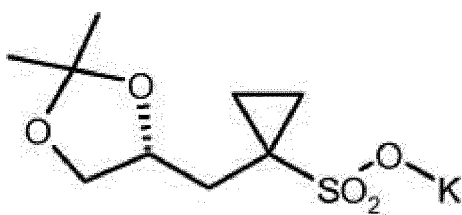
(R)-7' ;
