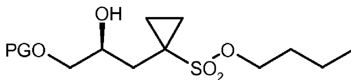
(S)-9
