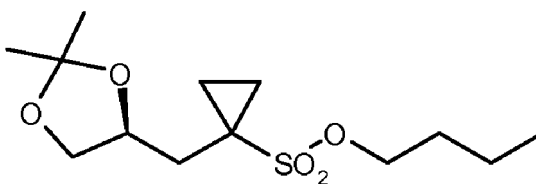
(S)-6
