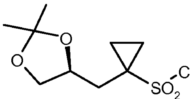
(S)-10
