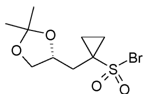
35 ((R)-10-Br
