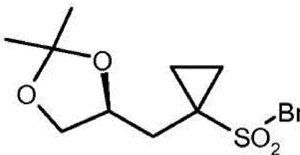
(S)-10-Br
