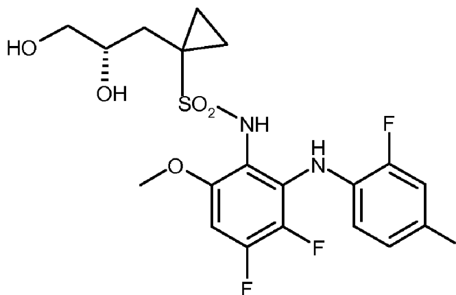
(S)-14.
