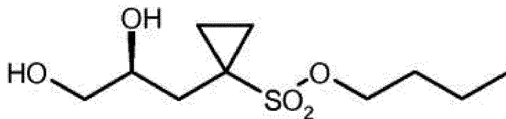
(S)-5
