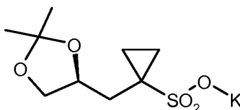
(S)-7'
