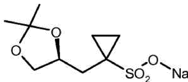
(S)-7
