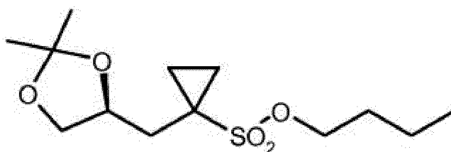
(S)-6;
