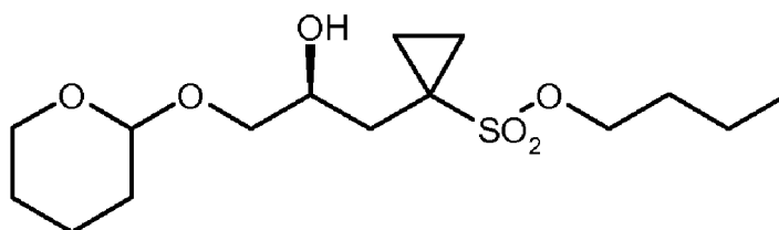
(S)-9b ;
