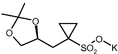
(S)-7' ;
