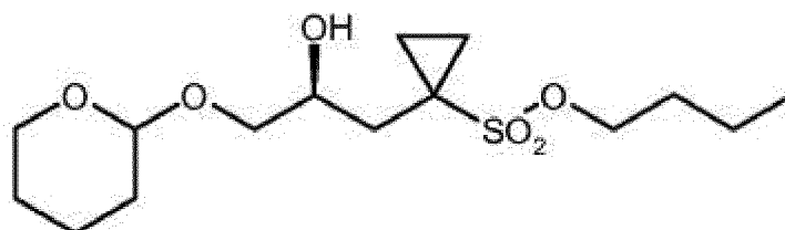
(S)-9b;
