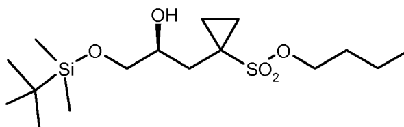
(S)-9a ;
