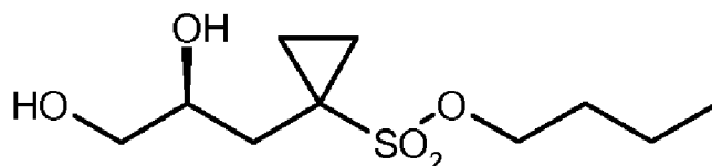
(S)-5
