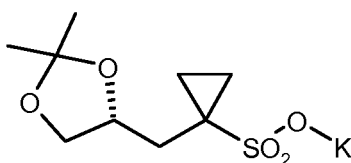
(R)-7'
