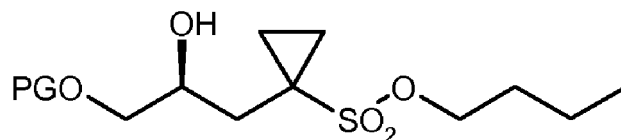
(S)-9 ;
