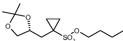
(R)-6
