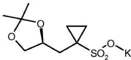
(S)-7' ;
