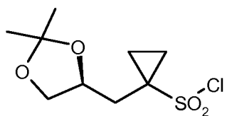
(S)-10
