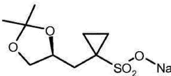
(S)-7
