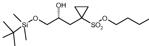
(R)-9a ;
