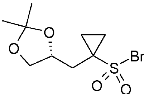
(R)-10-Br ;
