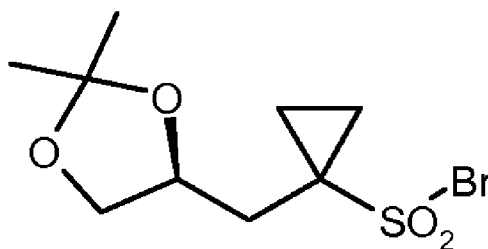
(S)-10-Br
