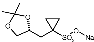
(R)-7
