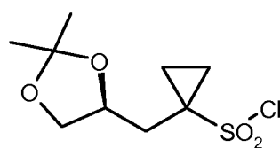
30 (S)-10
