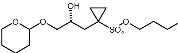
(R)-9b.
