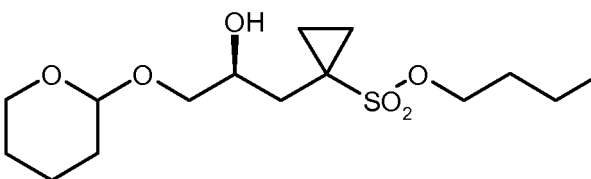
(S)-9b ;
