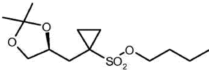
(S)-6
