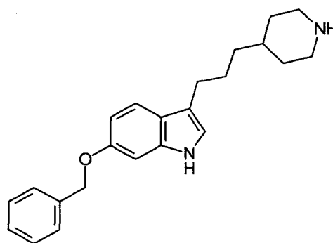
homo-6-BOIP
