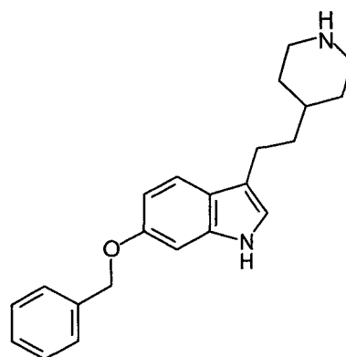
6-BOIP
