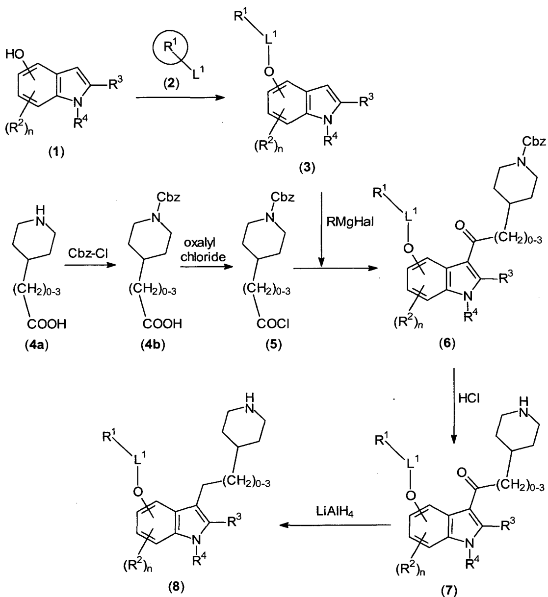
Scheme 2: Synthesis of the compounds of formula (I), route B.
