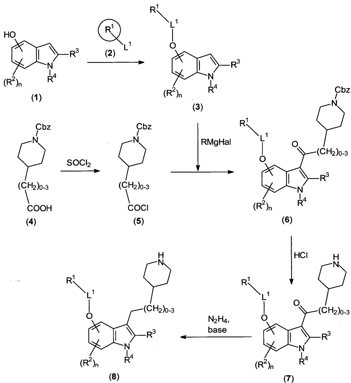
Scheme 1: Synthesis of the compounds of formula (I), route A.
