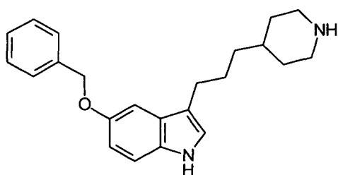
homo-5-BOIP
