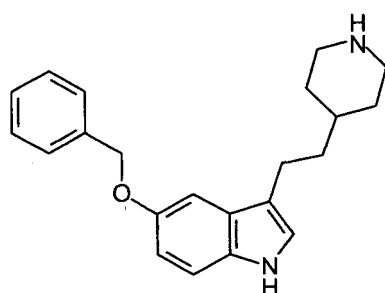
5-BOIP
