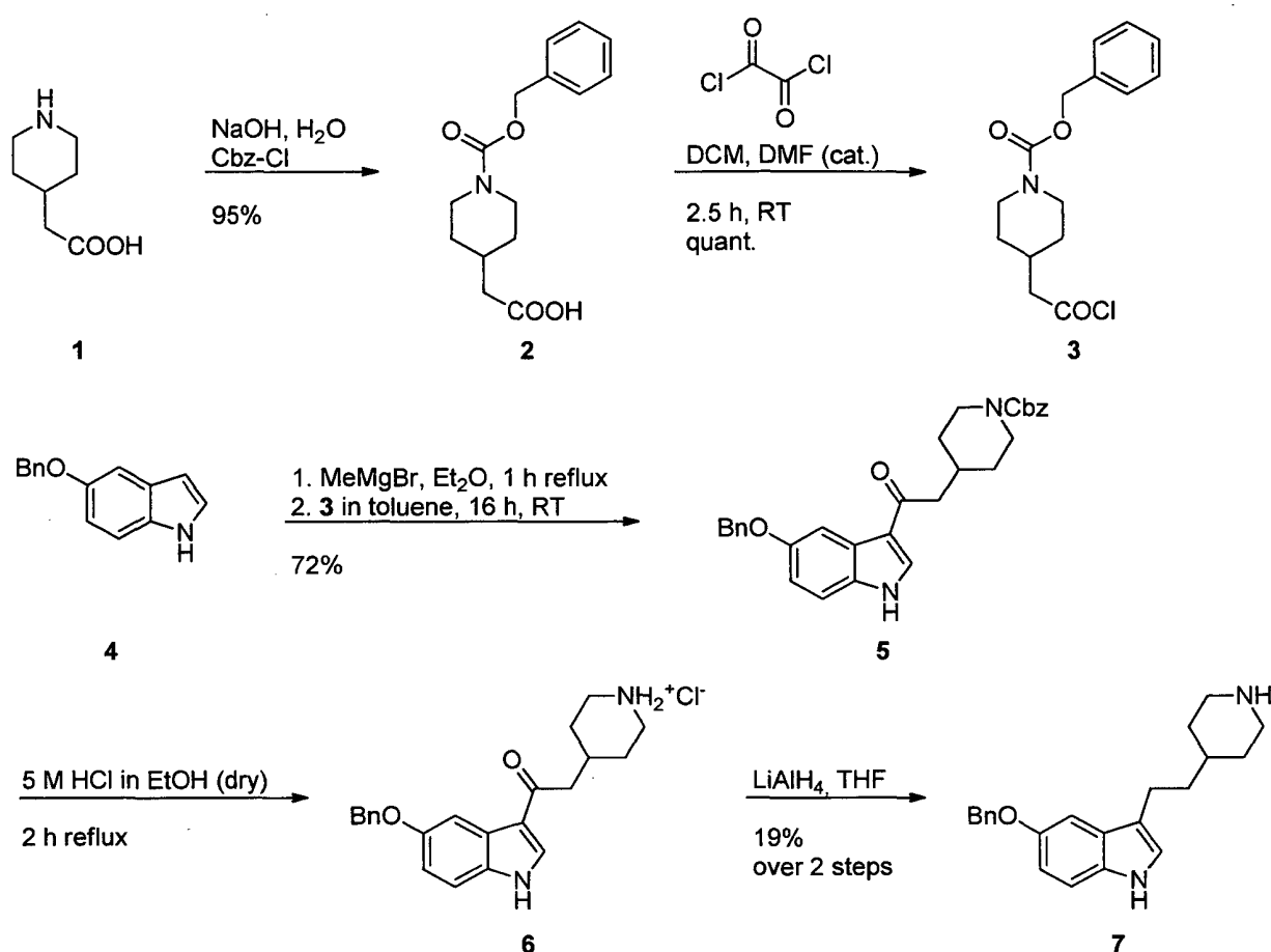
Scheme 4: Synthesis of 5-benzyloxyindalpine (5-BOIP), route B.
