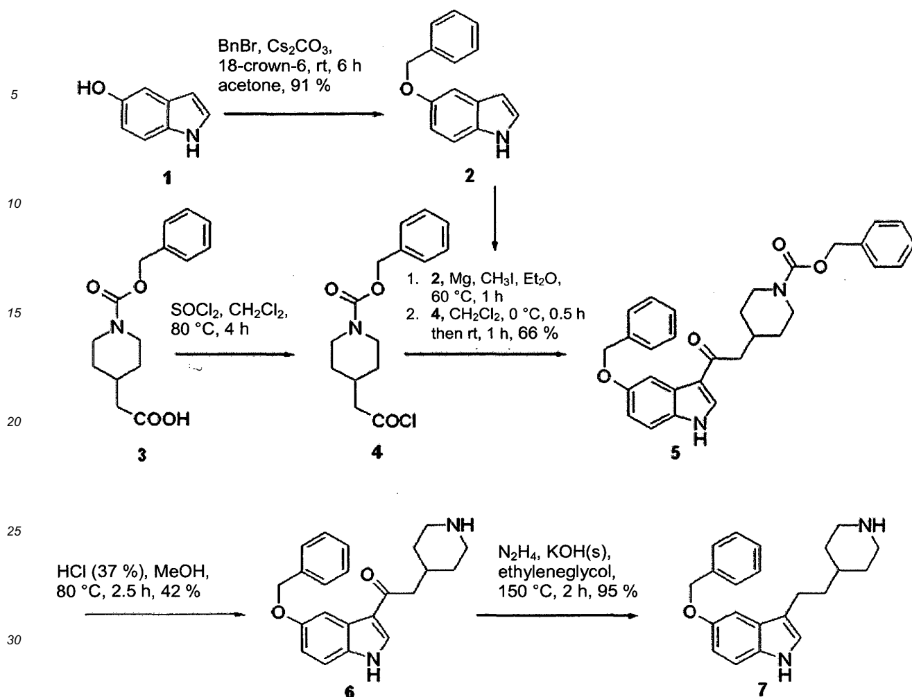
Scheme 3: Synthesis of 5-benzyloxyindalpine (5-BOIP), route A.
