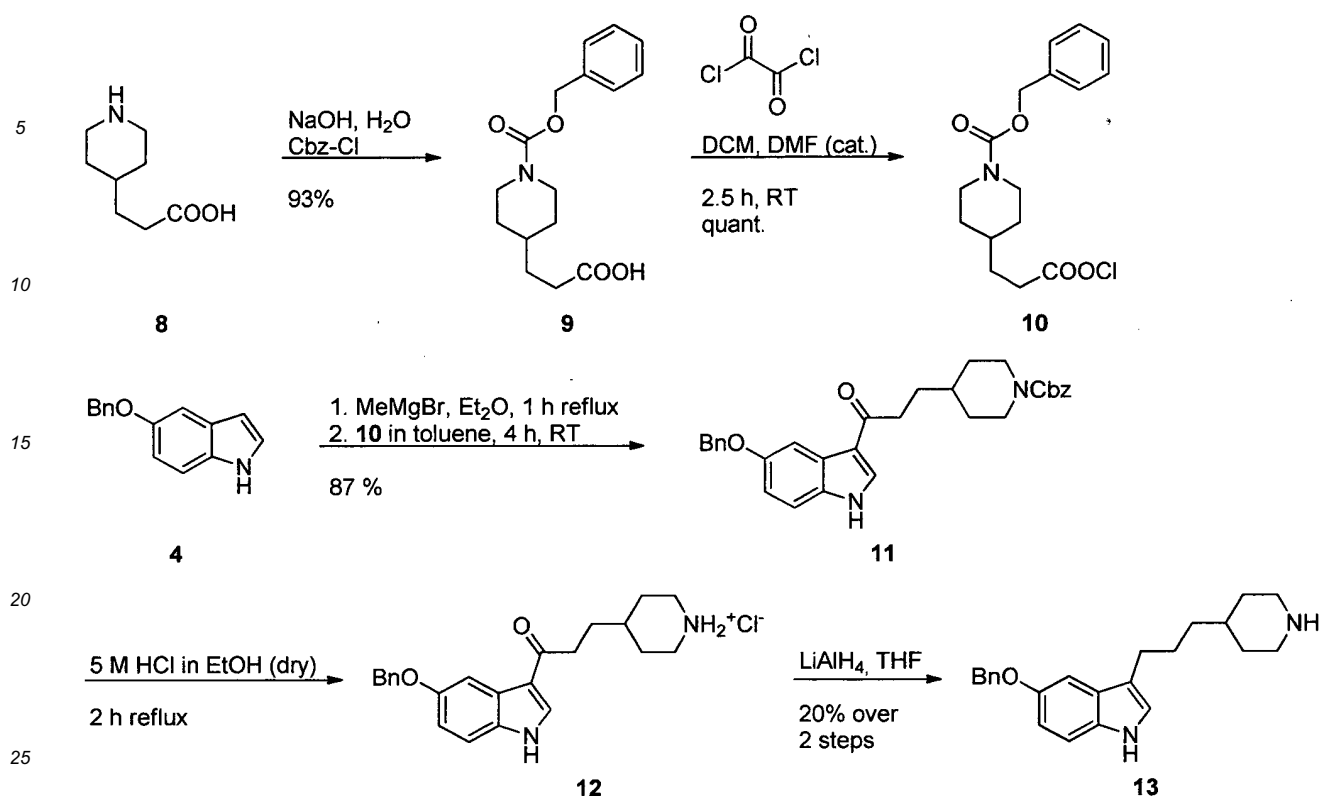
Scheme 5: Synthesis of homo-5-benzyloxyindalpine (homo-5-BOIP).
