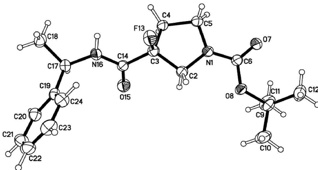
Figure 1. The X-ray crystal structure of compound (XVIII)
