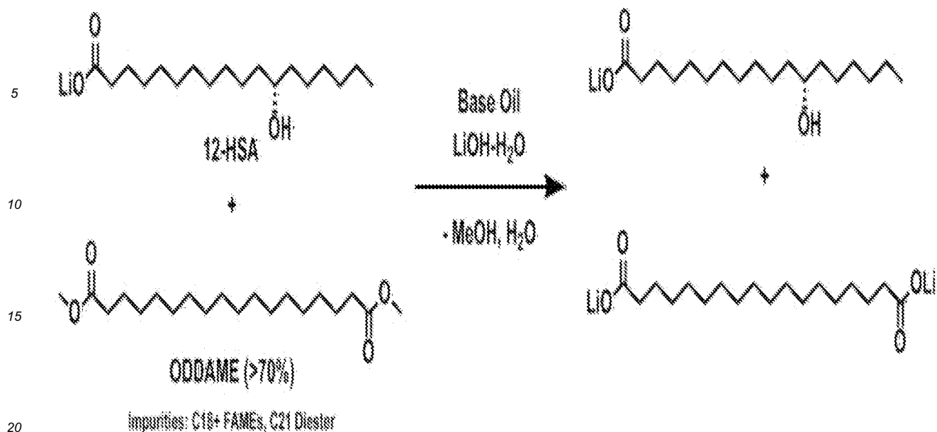
Figure 2. Reaction of ODDAME with 12-HSA as complexing agent.
