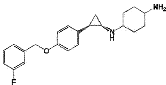
Example 65: N1-((trans)-2-(4-((4-fluorobenzyl)oxy)phenyl)cyclopropyl)cyclohexane-1,4-diamine
