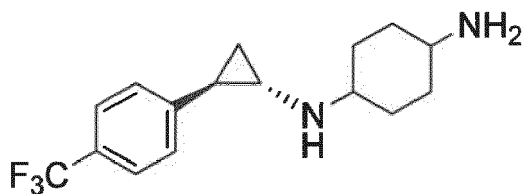
Example 77: N1-((trans)-2-(4-methoxyphenyl)cyclopropyl)cyclohexane-1,4-diamine
