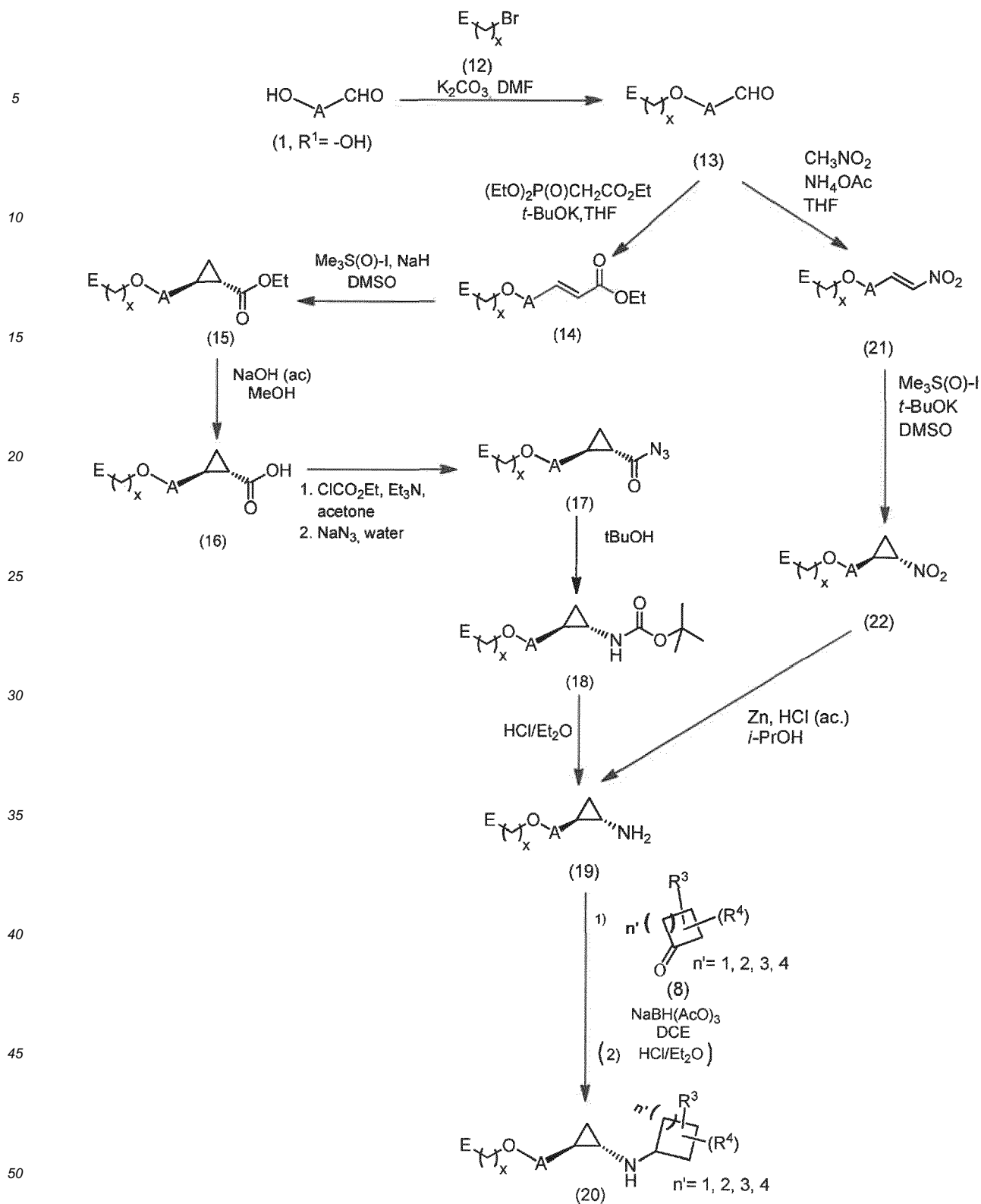
SCHEME 3: DCE (Dichloroethane), DMF (N,N-dimethylformamide), DMSO (Dimethyl sulfoxide), THF (Tetrahydrofuran)
