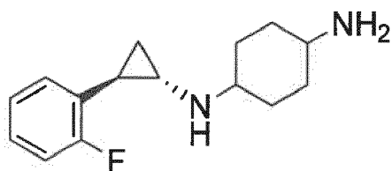
Example 79: N1-((trans)-2-(3,4-difluorophenyl)cyclopropyl)cyclohexane-1,4-diamine
