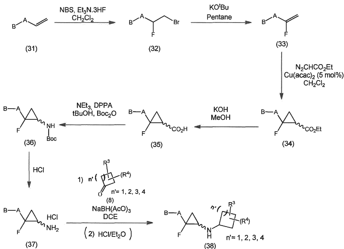
SCHEME 6: \text{Boc}_2\text{O} (Di- tert -butyl dicarbonate), DCE (Dichloroethane), DPPA (Diphenylphosphoryl azide), \text{Cu}(\text{acac})_2 (Copper(II) acetylacetonate), NBS (N-Bromosuccinimide).
