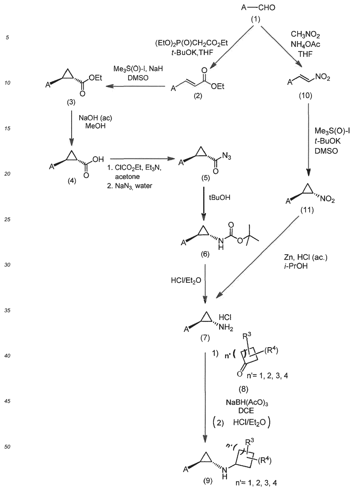
SCHEME 2: DCE (Dichloroethane), DMSO (Dimethyl sulfoxide), THF (Tetrahydrofuran). aq = aqueous.
