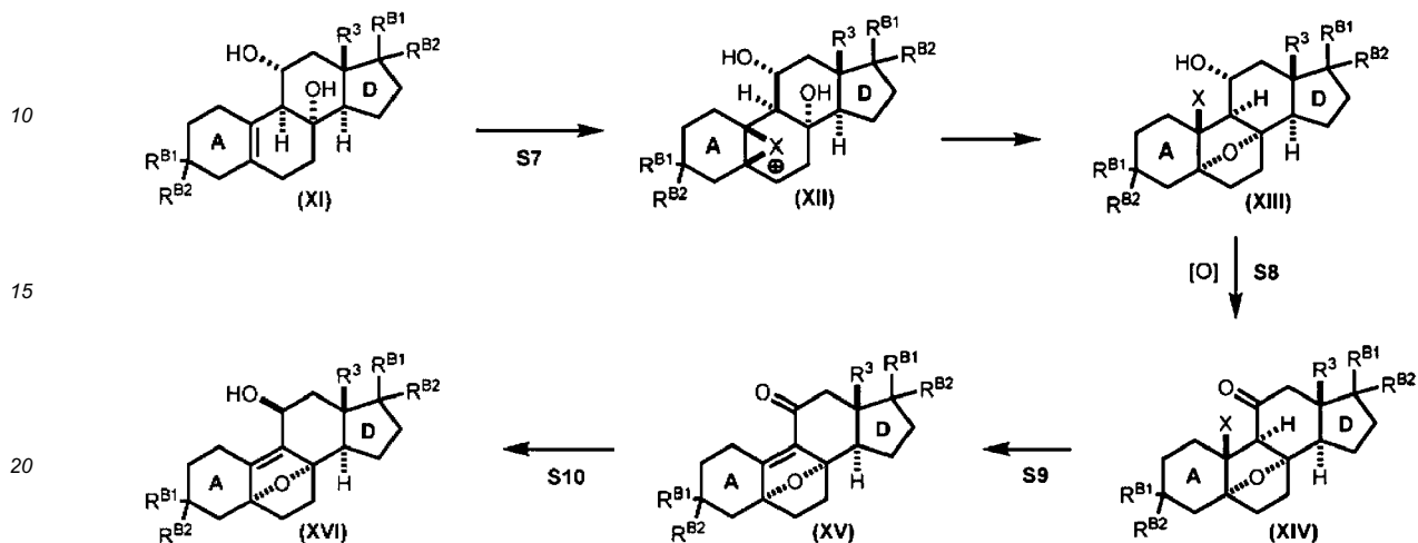
Scheme 6.
