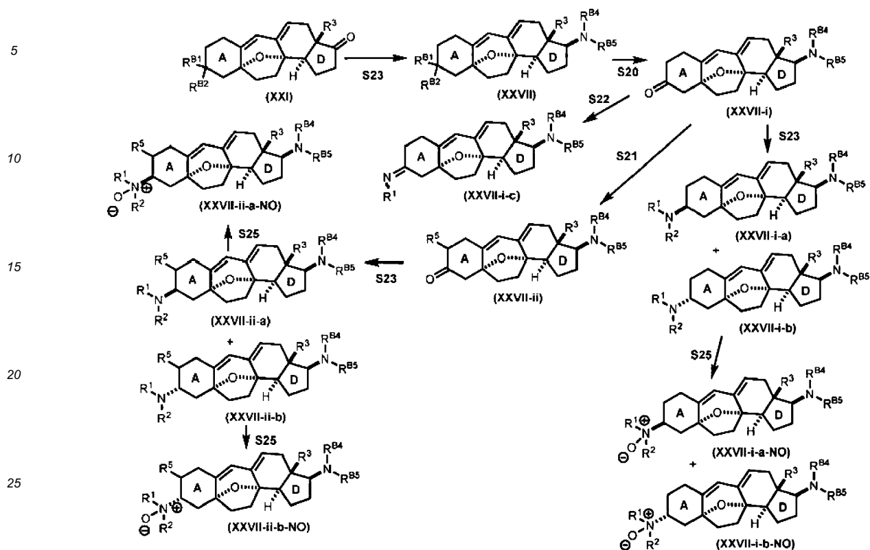
Scheme 13.
