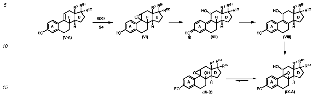
Scheme 4.
