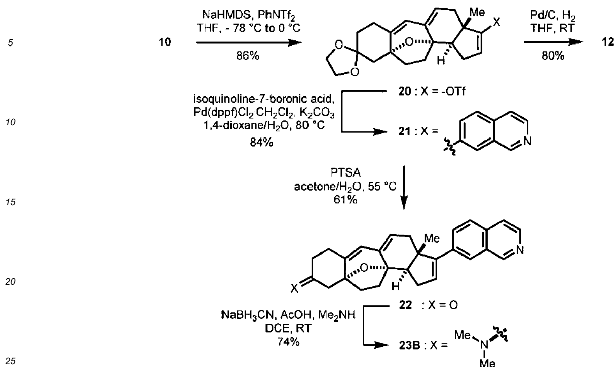
Scheme 2-1.
