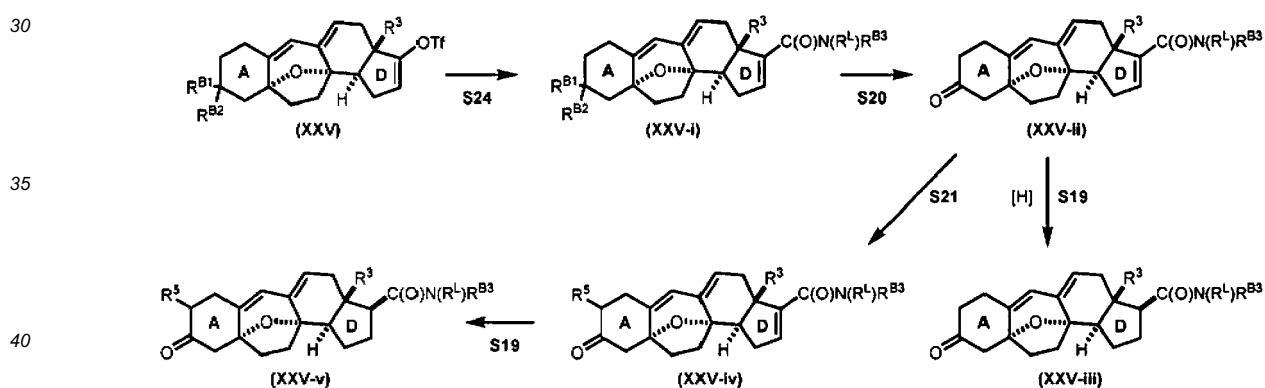
Scheme 11.
