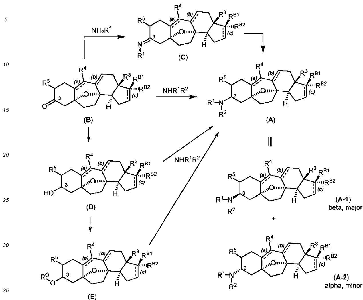
Scheme 1.
