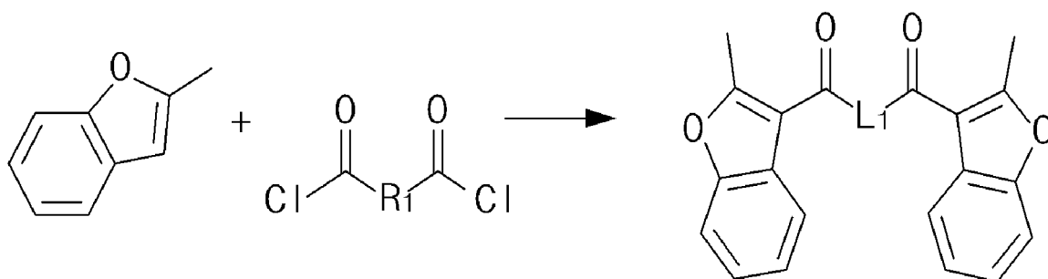
<Reaction Scheme 3>
