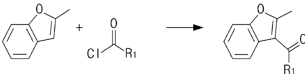
<Reaction Scheme 2>
