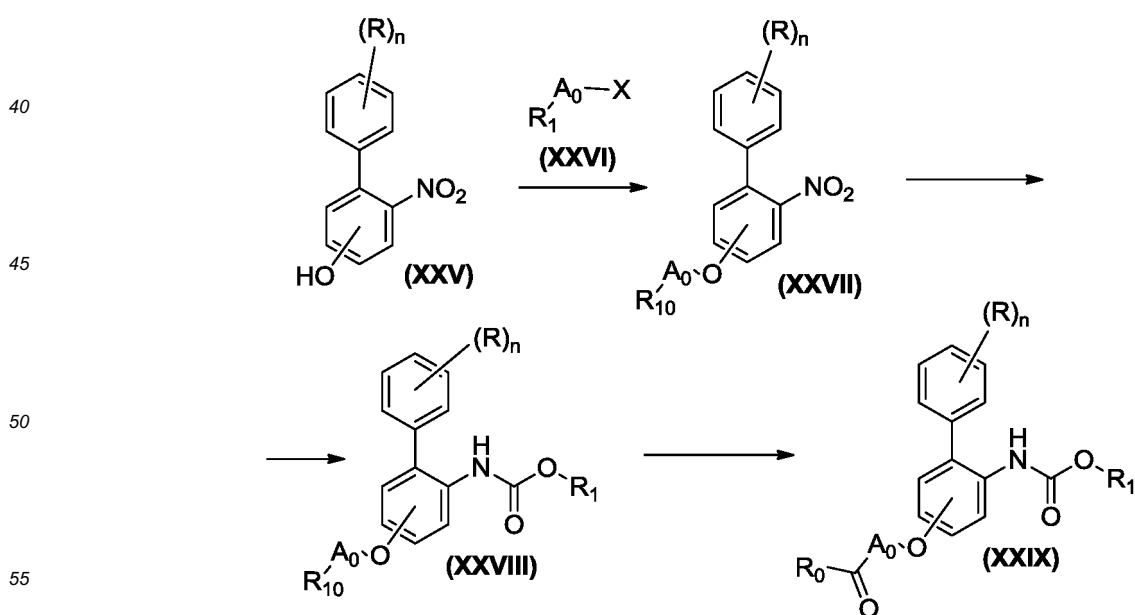
Scheme 6
