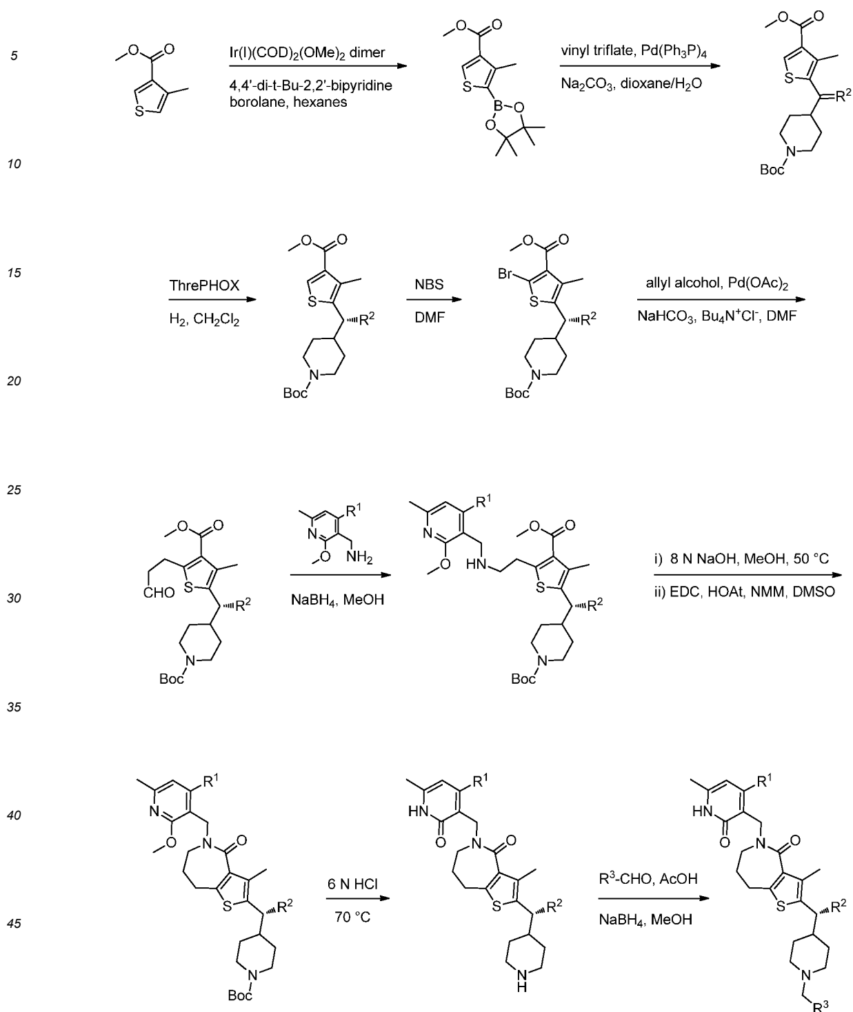
Scheme 1: Synthesis of Compounds of Formula (I).
