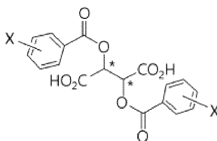
[Chemical Formula 1]
