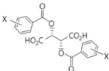
[Chemical Formula 3]
