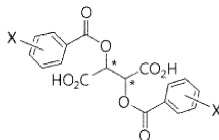
[Chemical Formula 1]
