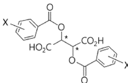
25 [Chemical Formula 1]
