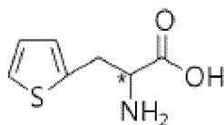
[Chemical Formula 4]
