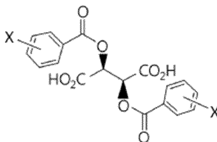
45 [Chemical Formula 2]
