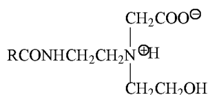
(MONO)ACETATE
