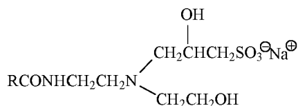
AMPHOTERIC SULFONATE
