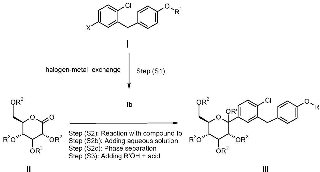
Scheme 1: Overview of the reaction steps for the synthesis of compound III
