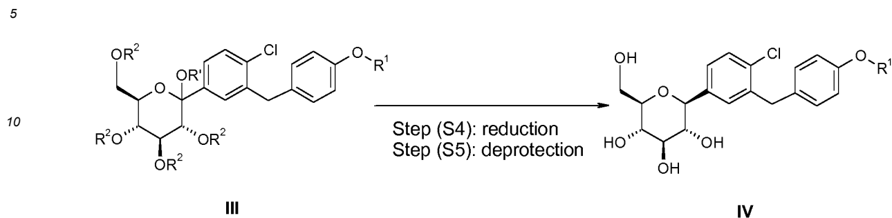
Scheme 2: Reduction and optional deprotection of compound III
