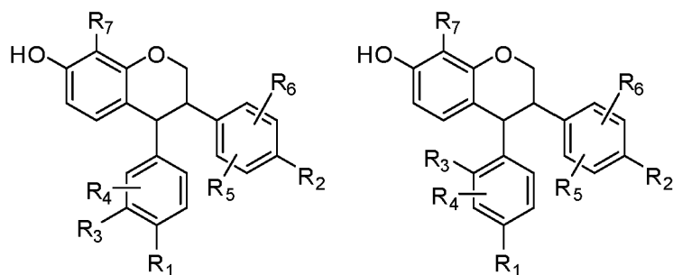
Formula (III-a)
