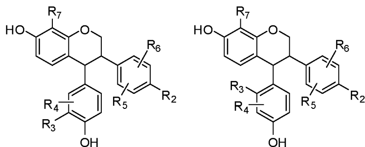
Formula (IV-a)
