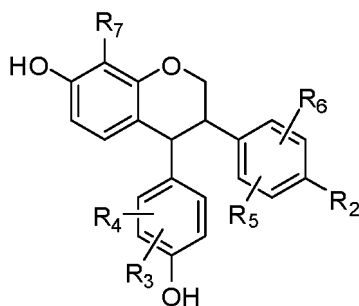
Formula (IV).
