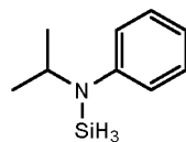
N-phenyl-N-isopropylaminosilane
