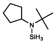
N-tert-butyl-N-cyclopentylaminosilane,
