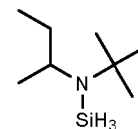
N-sec-butyl-N-tert-butylaminosilane
