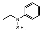
N-ethyl-N-phenylaminosilane
