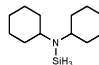
N,N-dicyclohexylaminosilane
