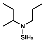
N-sec-butyl-N-n-propylaminosilane,
