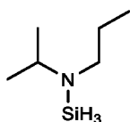
N-n-propyl-N-isopropylaminosilane,
