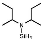
N,N-di-sec-butylaminosilane
