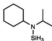
N-cyclohexyl-N-isopropylaminosilane,
