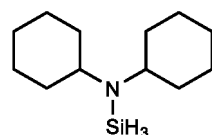
N,N-dicyclohexylaminosilane,
