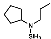
N-cyclopentyl-N-n-propylaminosilane,
