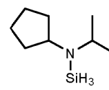
N-cyclopentyl-N-isopropylaminosilane
