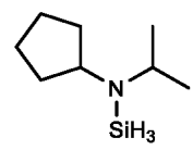
N-cyclopentyl-N-isopropylaminosilane,
