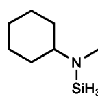
N-cyclohexyl-N-methylaminosilane,
