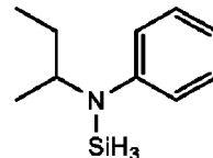
N-sec-butyl-N-phenylaminosilane,
