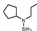
N-cyclopentyl-N-n-propylaminosilane
