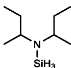
N,N-di-sec-butylaminosilane,
