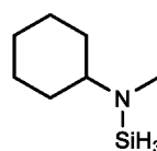
N-ethyl-N-cyclohexylaminosilane,
