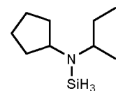
N-sec-butyl-N-cyclopentylaminosilane
