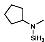
N-methyl-N-cyclopentylaminosilane,
