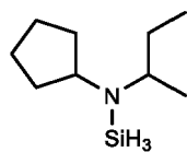
N-sec-butyl-N-cyclopentylaminosilane,
