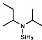
N-sec-butyl-N-isopropylaminosilane,
