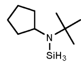
N-tert-butyl-N-cyclopentylaminosilane
