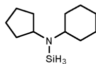
N-cyclohexyl-N-cyclopentylaminosilane
