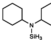
N-sec-butyl-N-cyclohexylaminosilane,
