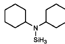
N,N-dicyclohexylaminosilane,
