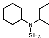
N-sec-butyl-N-cyclohexylaminosilane
