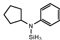
N-cyclopentyl-N-phenylaminosilane
