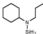
N-cyclohexyl-N-n-propylaminosilane
