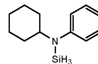
N-cyclohexyl-N-phenylaminosilane
