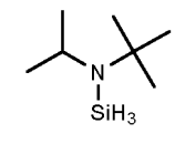
N-tert-butyl-N-iso-propylaminosilane
