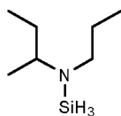
N-sec-butyl-N-n-propylaminosilane
