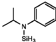
N-phenyl-N-isopropylaminosilane,
