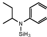
N-sec-butyl-N-phenylaminosilane
