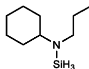
N-cyclohexyl-N-n-propylaminosilane,
