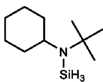
N-tert-butyl-N-cyclohexylaminosilane,
