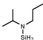
N-n-propyl-N-isopropylaminosilane
