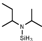
N-sec-butyl-N-isopropylaminosilane
