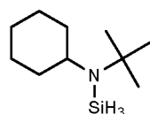
N-tert-butyl-N-cyclohexylaminosilane
