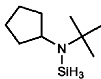
N-tert-butyl-N-cyclopentylaminosilane,
