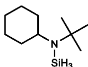
N-tert-butyl-N-cyclohexylaminosilane,
