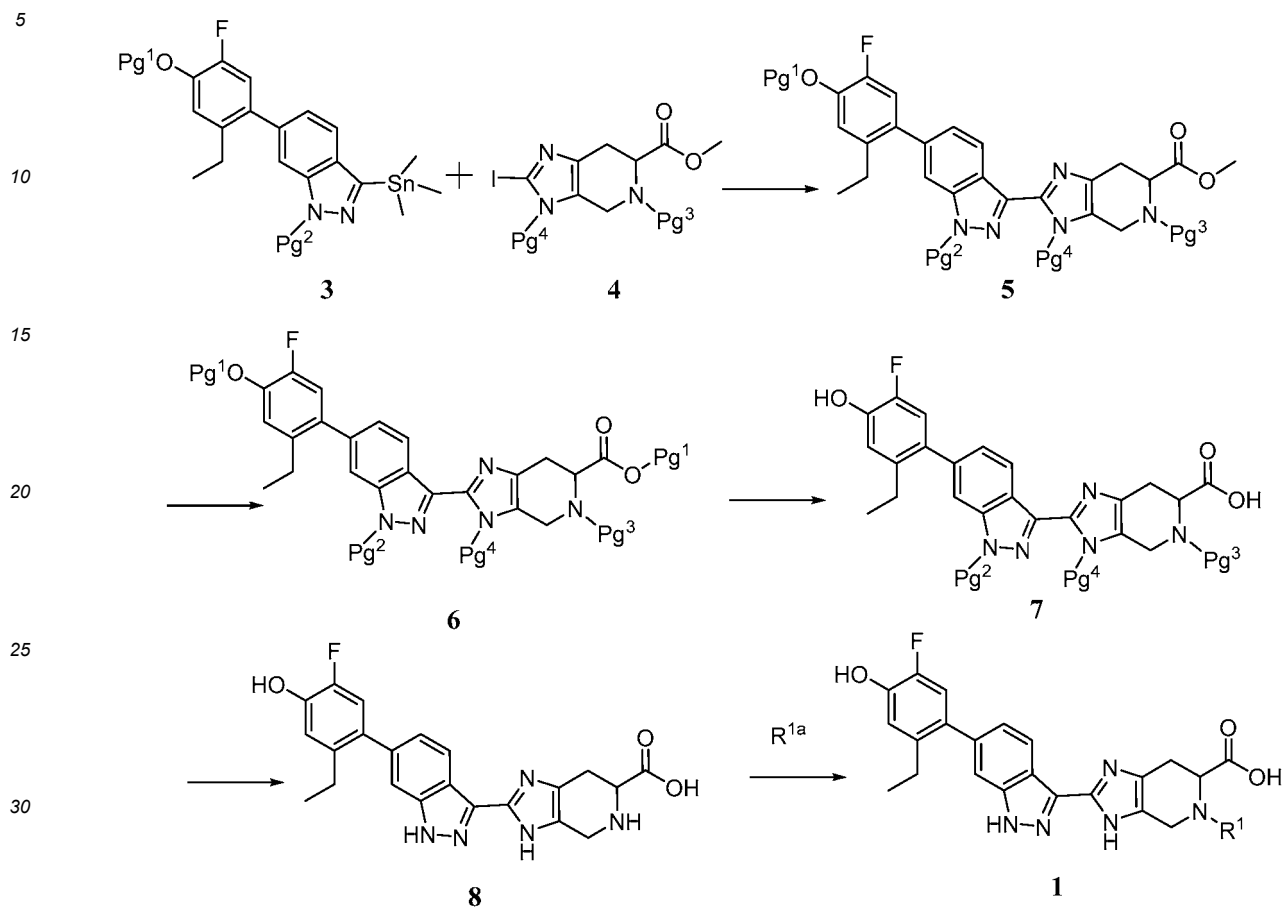
Scheme 2
