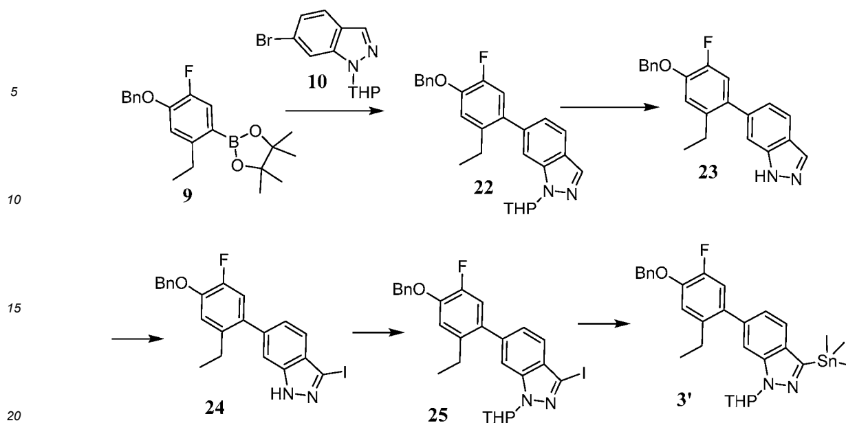
(a) 6-(4-(Benzyloxy)-2-ethyl-5-fluorophenyl)-1-(tetrahydro-2H-pyran-2-yl)-1H-indazole ( 22 )
