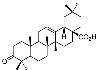
Oleanonic acid (OLN)
