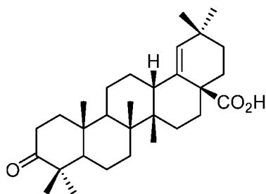
Moronic acid (MA)
