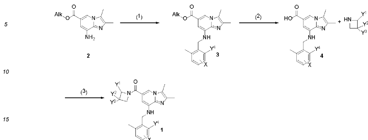
Reaction scheme 1
