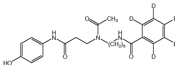
MPS-I Internal Standard
