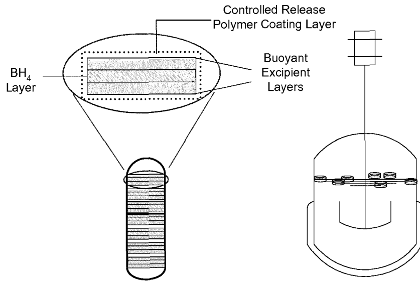
Schematic Diagram of Floating Dosage Form
