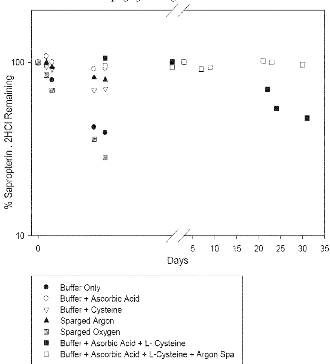
FIGURE 36 Stability of BH4 in pH 4 Buffer in the Presence and Absence of Antioxidants and Sparging with Argon
