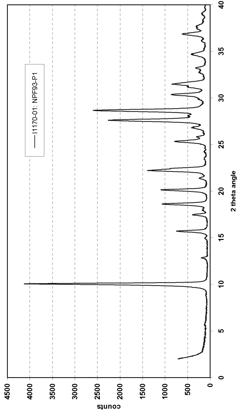
Figure 1 Powder X-ray Diffraction Pattern of (6R)-L-erythro-Tetrahydrobiopterin Dihydrochloride Form B
