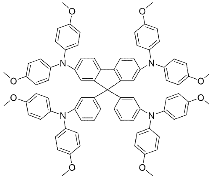
Spiro-OMeTAD
