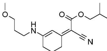
2-methylpropyl (2Z)-cyano{3-[(3-methoxypropyl)amino]cyclohex-2-en-1-ylidene}ethanoate
