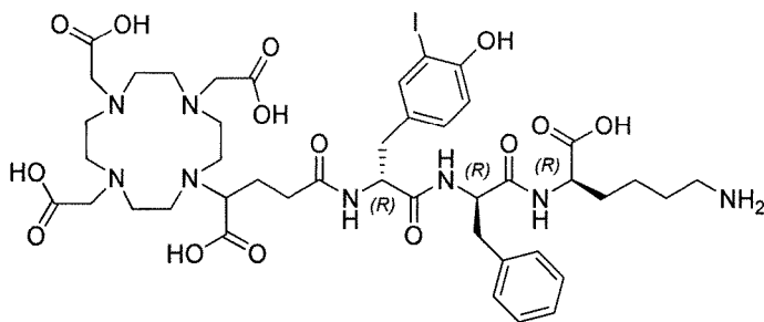
Chemical Formula: C_{43}H_{61}IN_8O_{14} Molecular Weight: 1040,91
