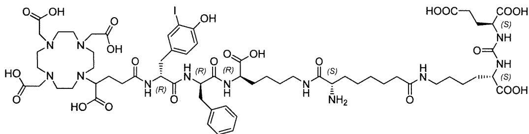
Chemical Formula: C_{63}H_{93}IN_{12}O_{23} Molecular Weight: 1513,40
