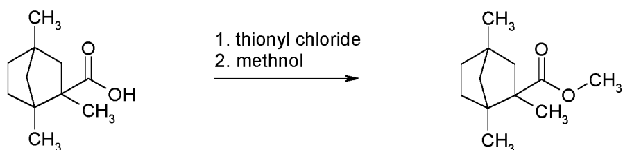
1,2,4-trimethyl-bicyclo[2.2.1] heptane-2-carboxylic acid
