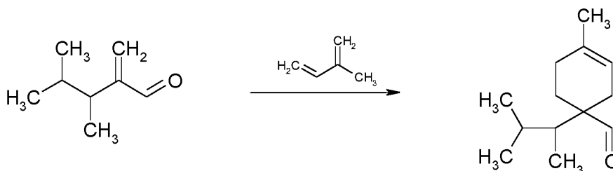
1-(1,2-dimethyl-propyl)-4-methyl -cyclohex-3-enecarbaldehyde
