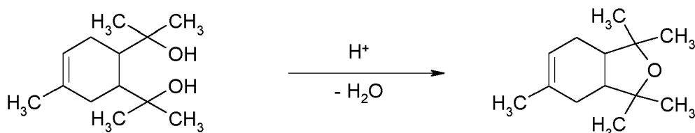
2-[6-(1-hydroxy-1-methyl-ethyl)-4-methyl-cyclohex-3-enyl]-propan-2-ol
