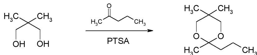
2,5,5-trimethyl-2-propyl -[1,3]dioxane
