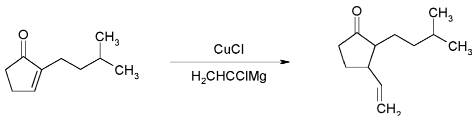
2-(3-methyl-butyl)- cyclopent-2-enone
