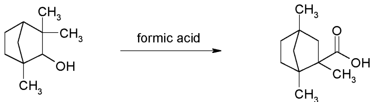
1,2,4-trimethyl-bicyclo[2.2.1] heptane-2-carboxylic acid
