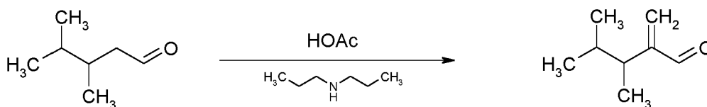
3,4-dimethyl-pentanal
