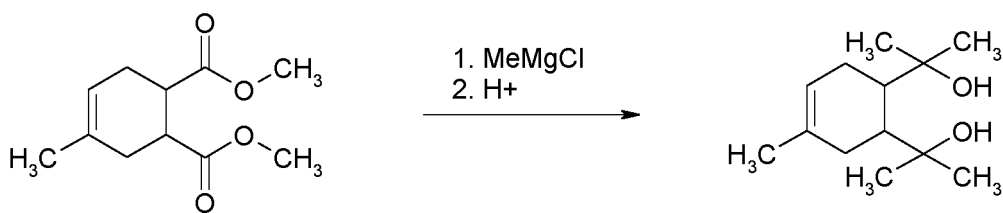
4-methyl-cyclohex-4-ene-1,2-dicarboxylic acid dimethyl ester
