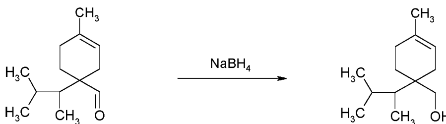
1-(1,2-dimethyl-propyl)-4-methyl -cyclohex-3-enecarbaldehyde
