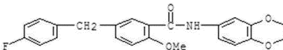
compound A
