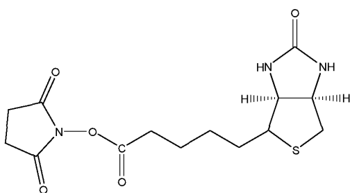
N-hydroxysuccinimide biotin
