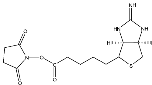
N-hydroxysuccinimide iminobiotin
