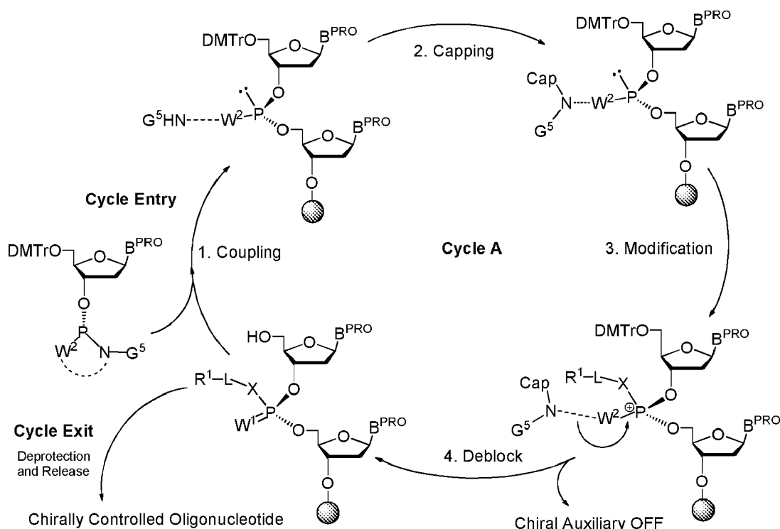
Scheme I. Synthesis of chirally controlled oligonucleotide.
