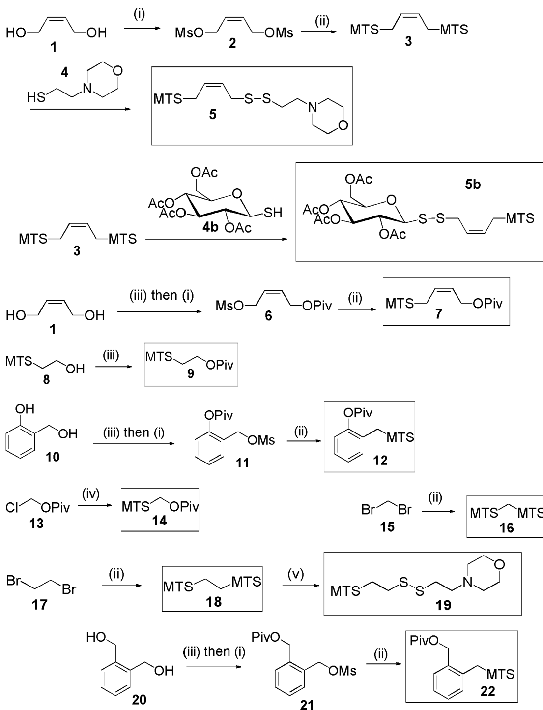
Scheme E-1. Synthesis of sulfurizing reagents.
