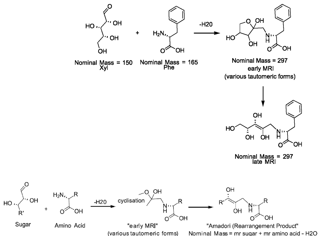
Reaction Scheme 1, Example of early Maillard reaction between xylose and phenylalanine
