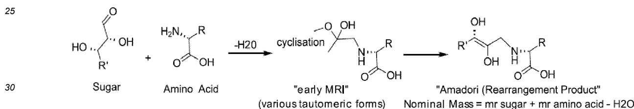
Reaction Scheme 2, General formation of Amadori products
