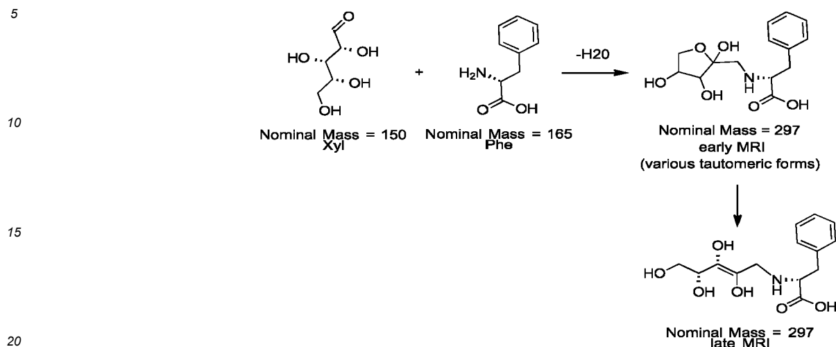
Reaction Scheme 1, Example of early Maillard reaction between xylose and phenylalanine
