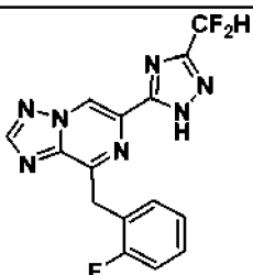
I-26
