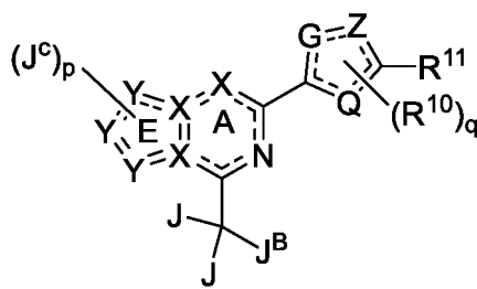
Formula IIA
