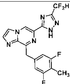
I-35
