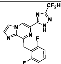
I-20
