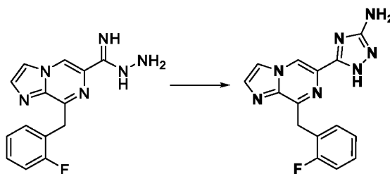
Compound I-57
