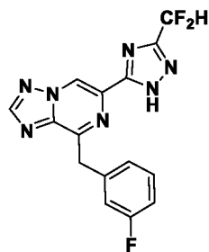
Compound I-21
