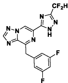
Compound I-25
