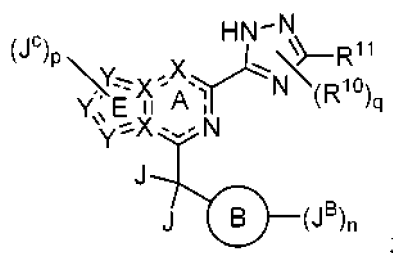
Formel III.
