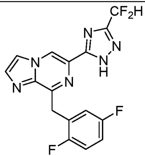
I-9
