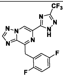
I-33
