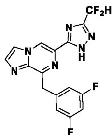
Compound I-30
