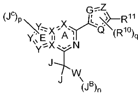
Formel I
