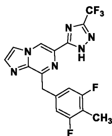
Compound I-34
