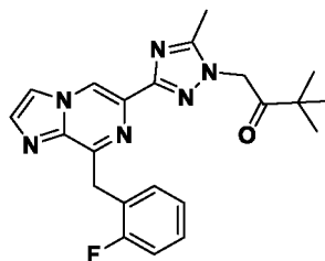
Compound I-48
