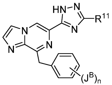
Formula VI
