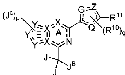
Formel IIA
