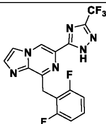
I-19
