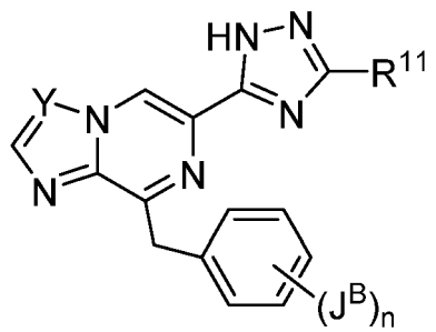
Formula V
