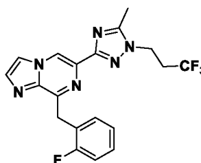
Compound I-54
