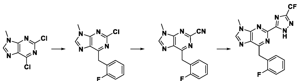
Compound I-37
