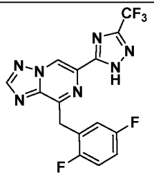
I-33
