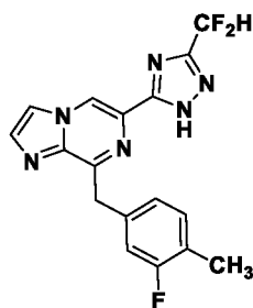
Compound I-28
