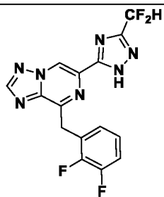
I-17
