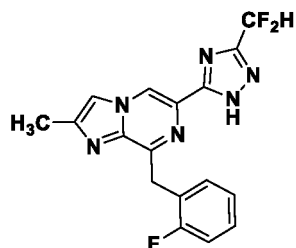
Compound I-32
