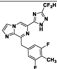
I-35
