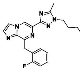
Compound I-56
