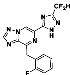
Compound I-26
