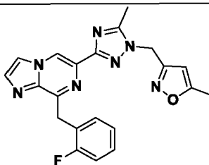
I-51
