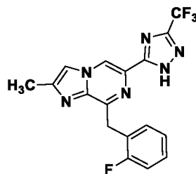
Compound I-31
