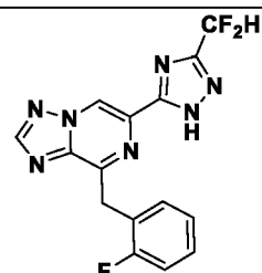
I-26
