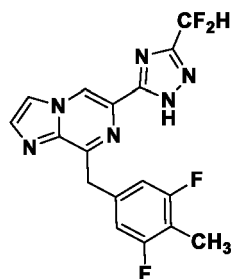
Compound I-35
