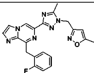
I-51
