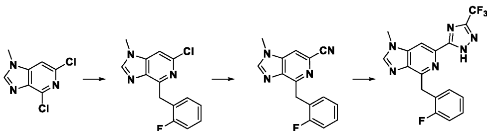
Compound I-36
