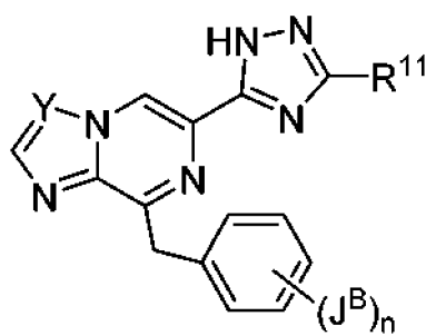
Formel V
