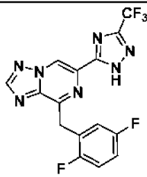
I-33
