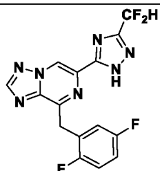
I-23
