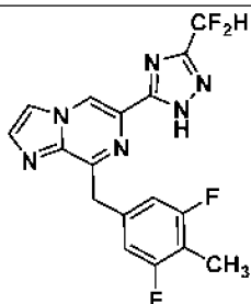
I-35
