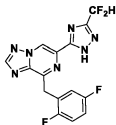
Compound I-23
