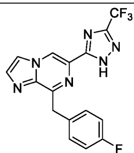
I-12
