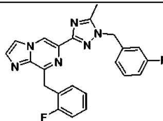
I-47
