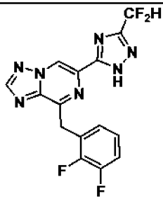
I-17
