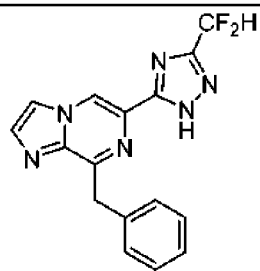
I-7
