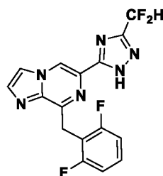
Compound I-20
