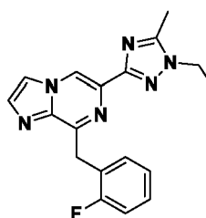
Compound I-53
