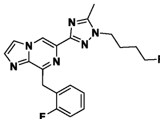
Compound I-50
