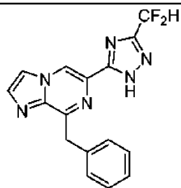
I-7
