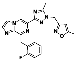
Compound I-51
