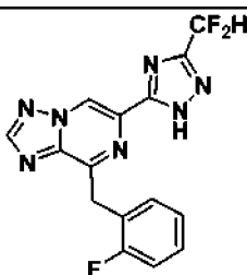
I-26
