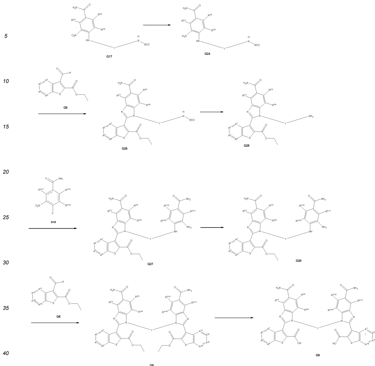
Scheme 6
