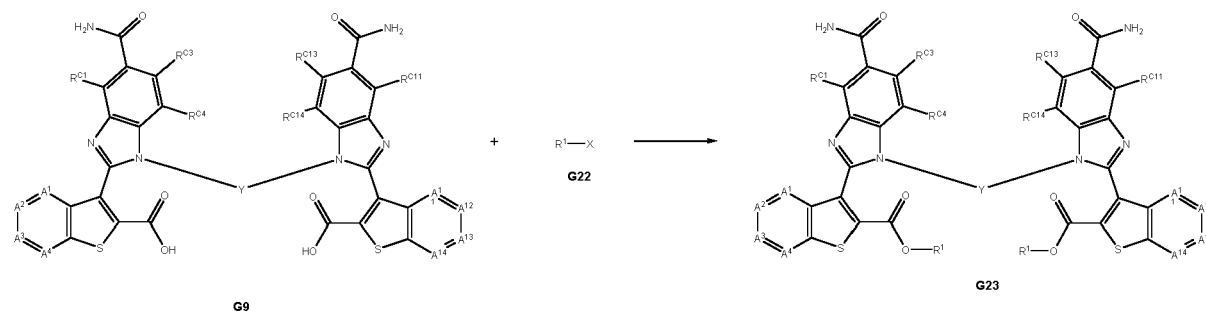
Scheme 5b
