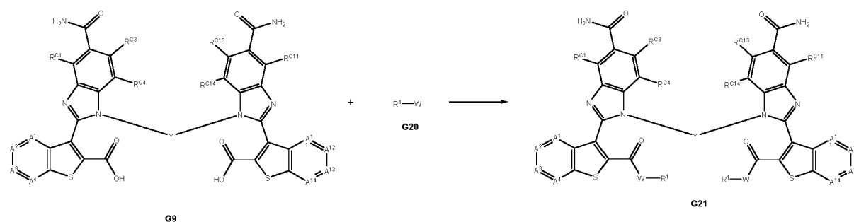
Scheme 5a
