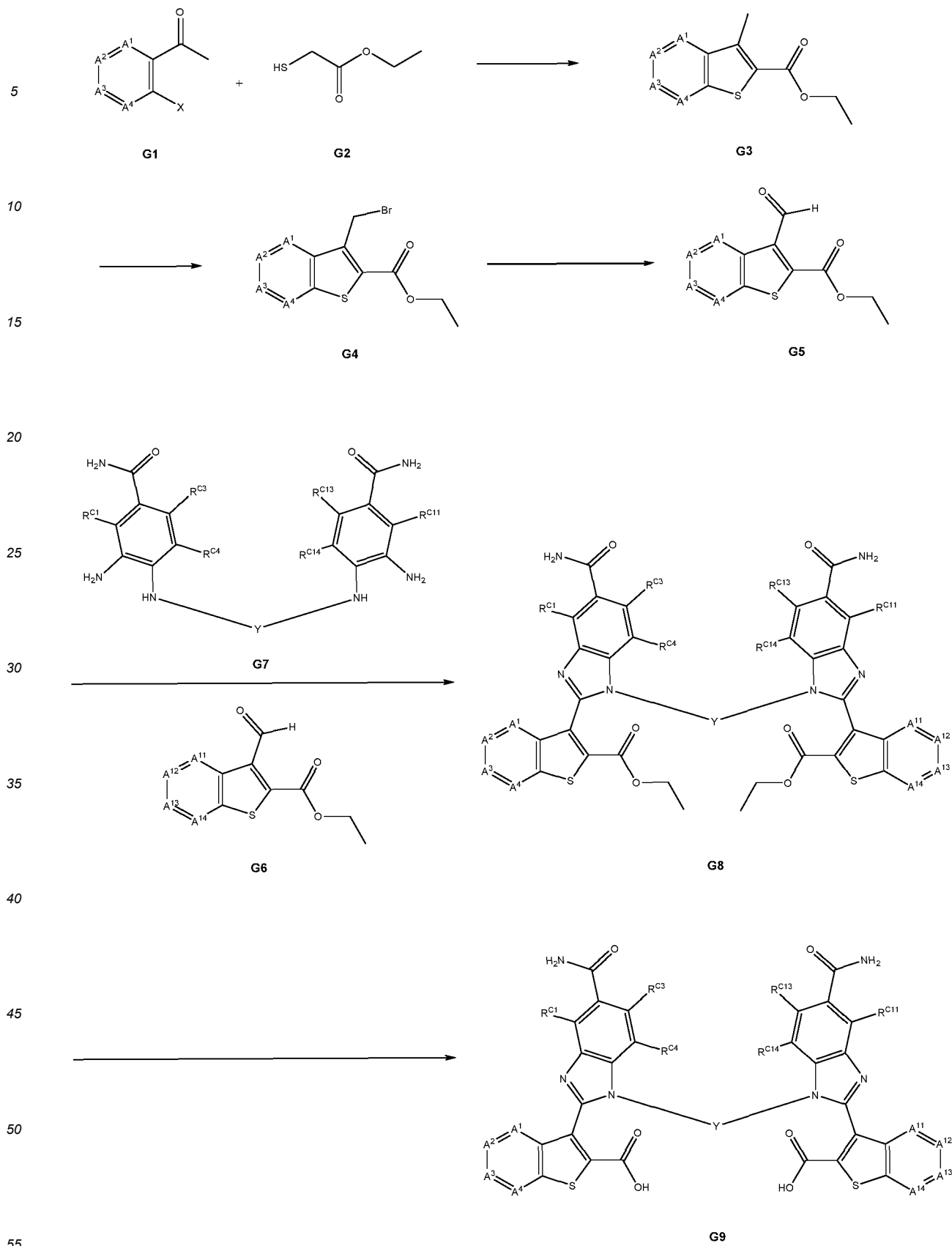
Scheme 1
