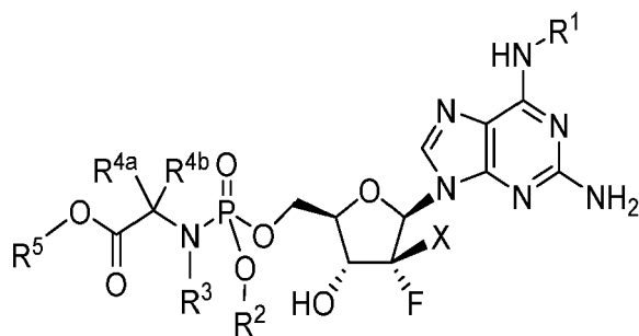
Formula III
