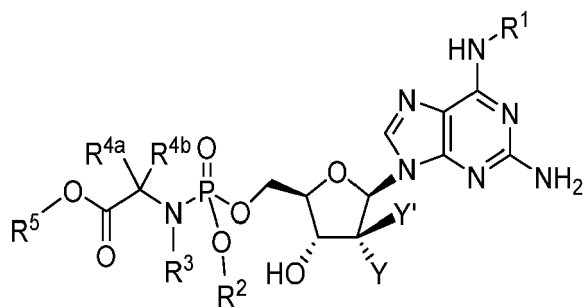
Formula V
