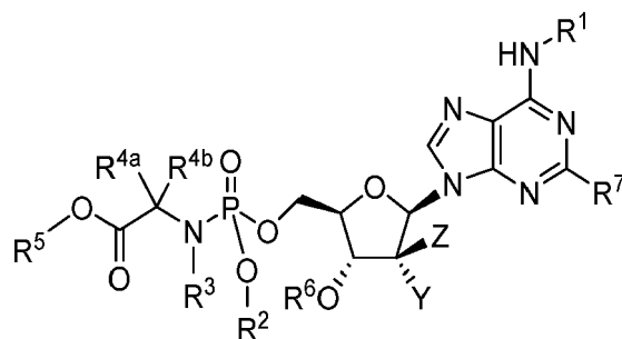
Formula VI
