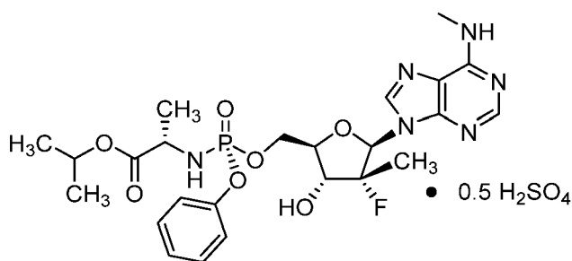
Compound 4B
