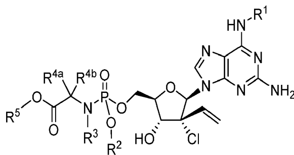
Formula IVd
