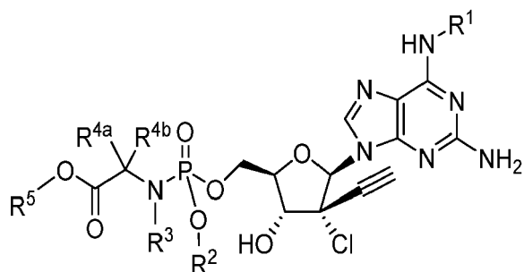
Formula IVe
