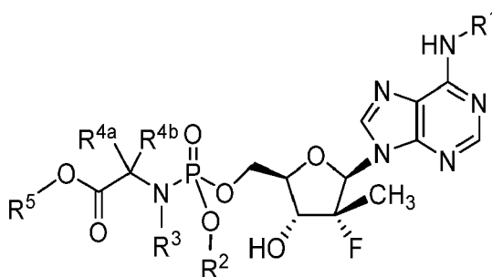
Formula II
