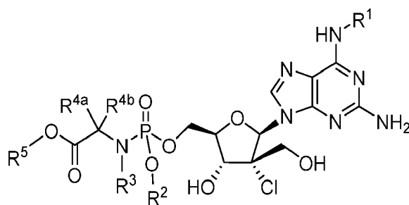
Formula IVf
