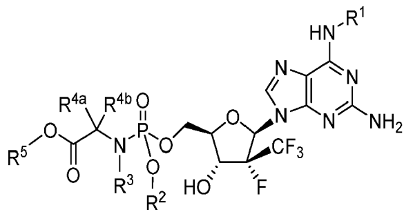
Formula IIIb
