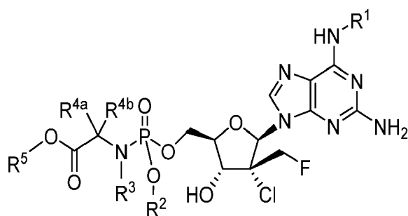
Formula IVa
