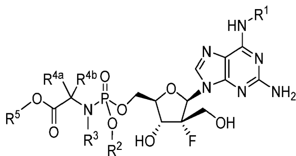
Formula IIIf
