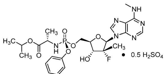
Compound 4A
