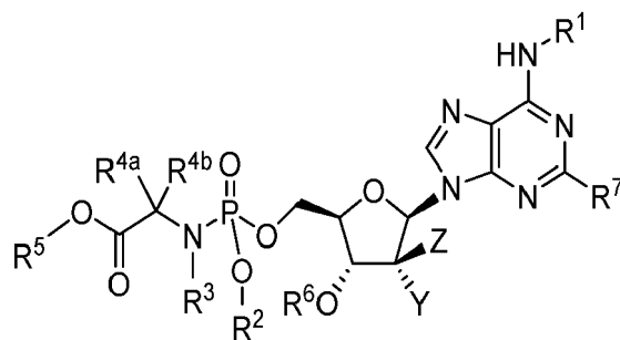
Formula VI
