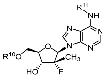
Formula X
