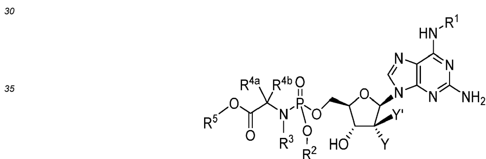
Formula V
