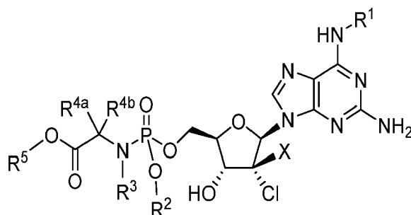
Formula IV
