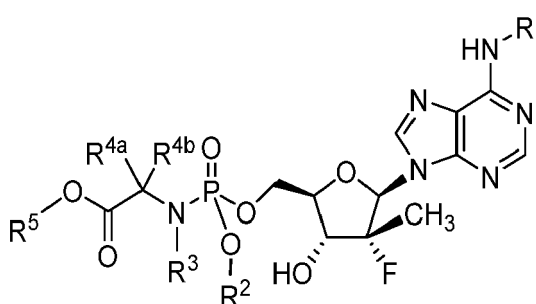
Formula II
