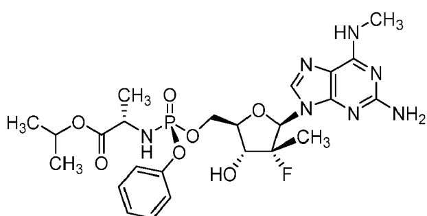
Compound 1A
