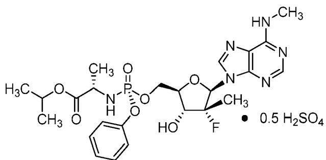
Compound 4B
