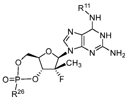
Formula IX'
