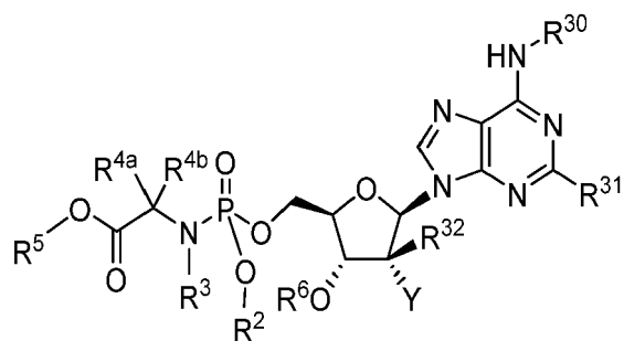
Formula XIII
