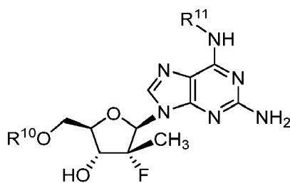
Formula IX
