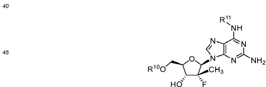
Formula IX
