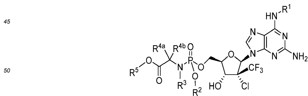
Formula IVb
