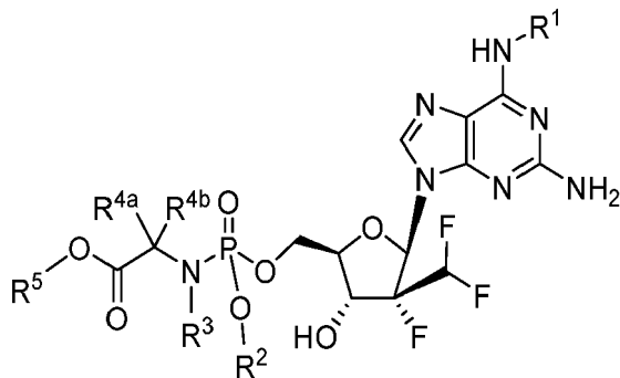
Formula IIIc
