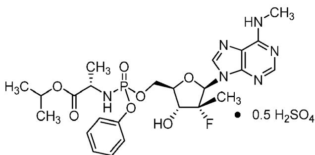
Compound 4
