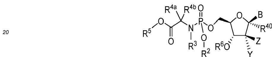
25 Formula VII
