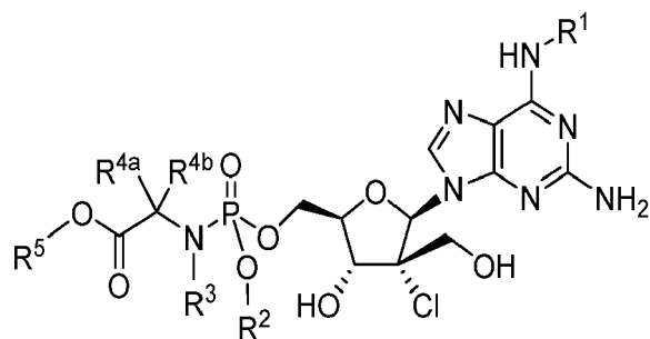
Formula IVf
