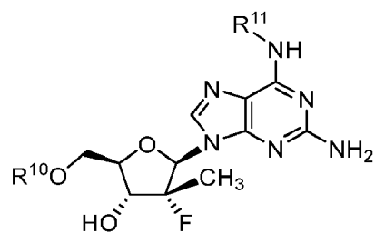
10 Formula IX
