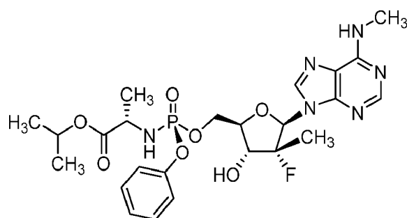
Compound 3A
