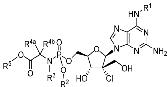
Formula IVf
