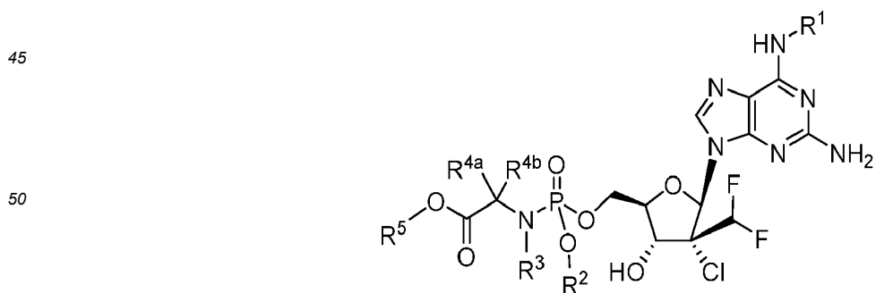
Formula IVc
