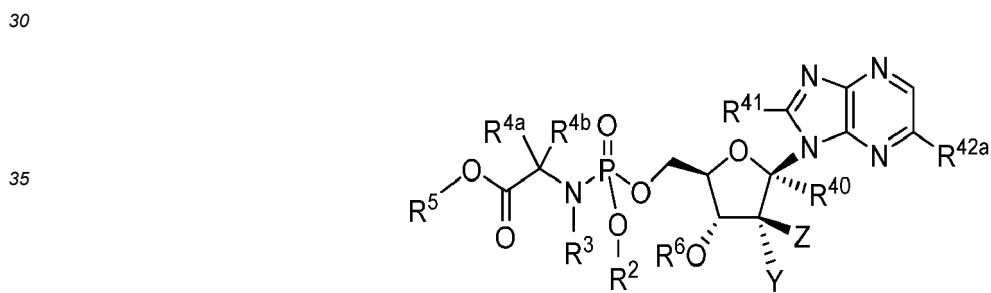
Formula VIIa
