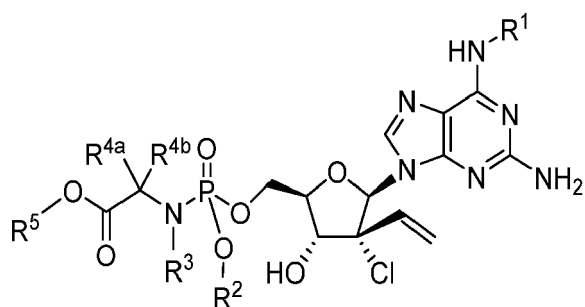
Formula IVd
