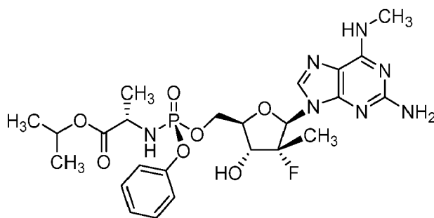
Compound 1A
