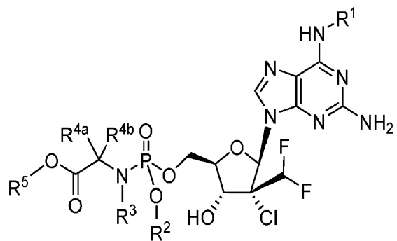
Formula IVc
