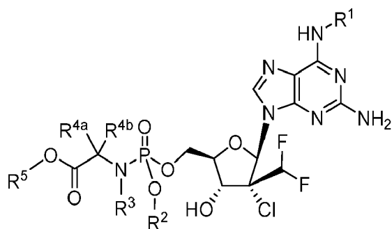
Formula IVc
