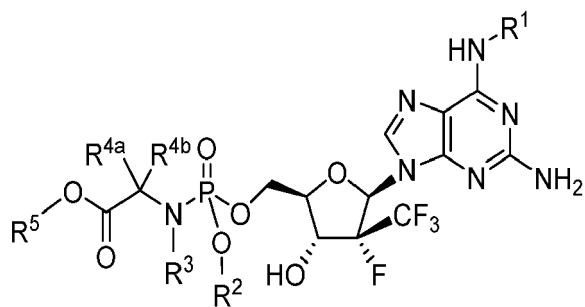
Formula IIIb
