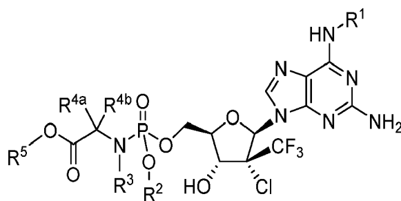
Formula IVb
