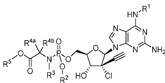
Formula IVe
