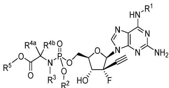
Formula IIIe
