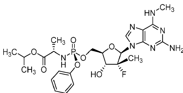
40 45 50 Compound 1A
