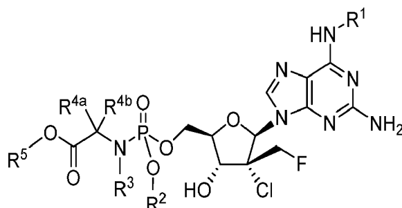
Formula IVa
