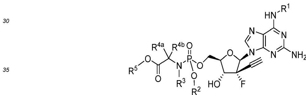
Formula IIIe
