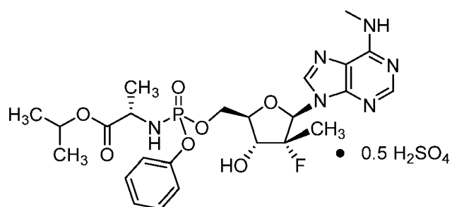
Compound 4
