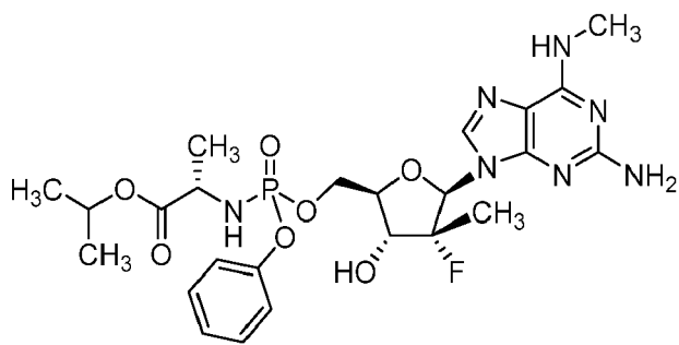
Compound 1
