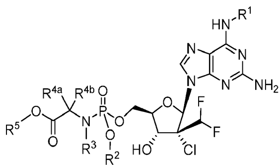
Formula IVc
