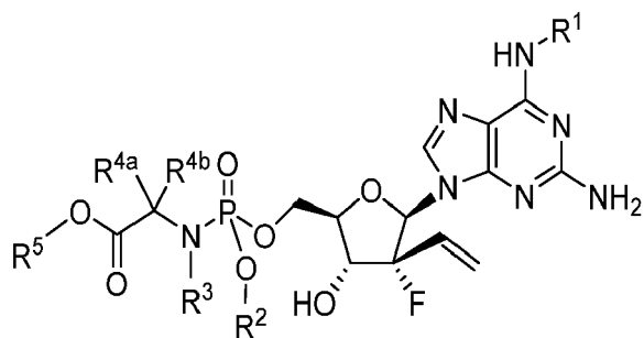
Formula IIId
