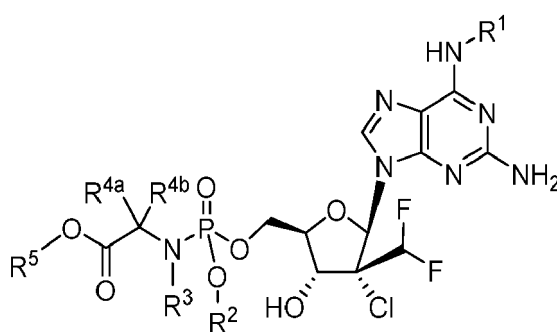
Formula IVc
