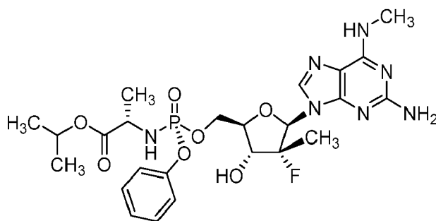
Compound 1B
