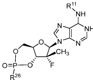
Formula X'
