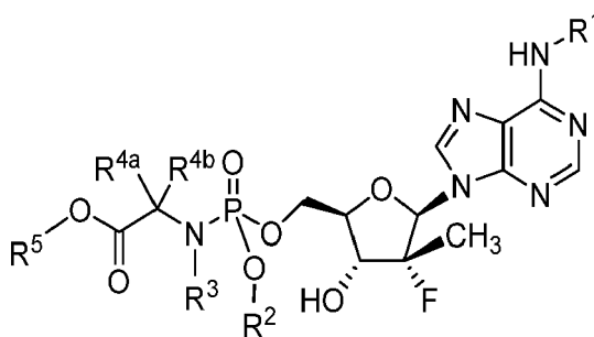
Formula II
