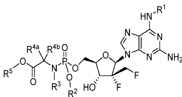
Formula IIIa
