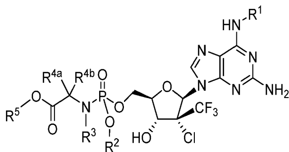
Formula IVb
