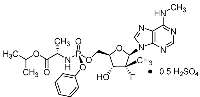
Compound 4A
