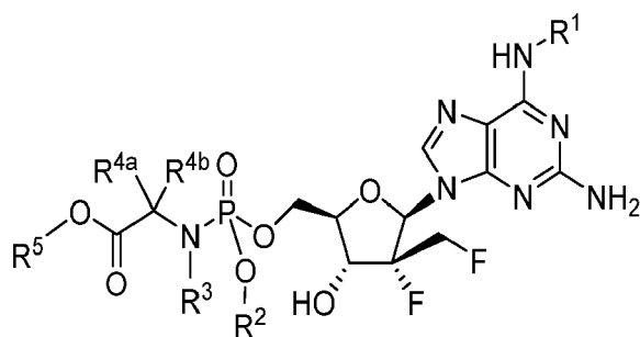
Formula IIIa
