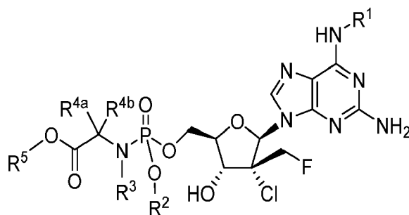
Formula IVa
