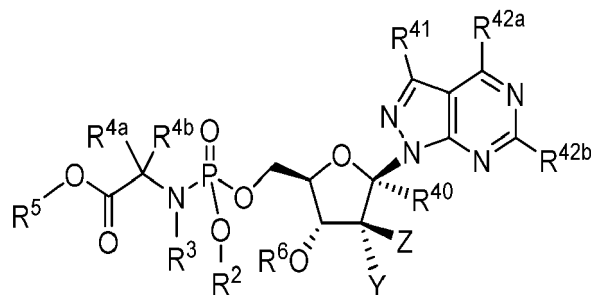
Formula VIIc
