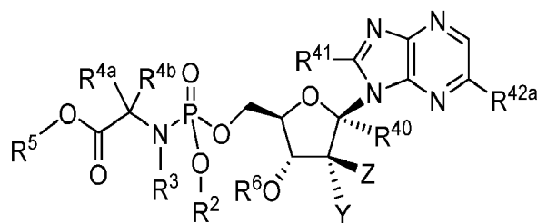
Formula VIIa
