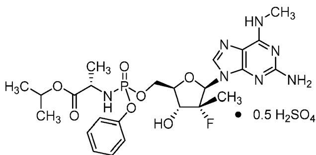
Compound 2
