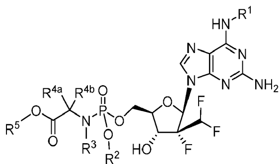
Formula IIIc
