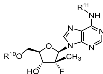
10 Formula X
