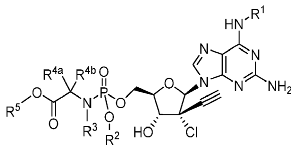
Formula IVe
