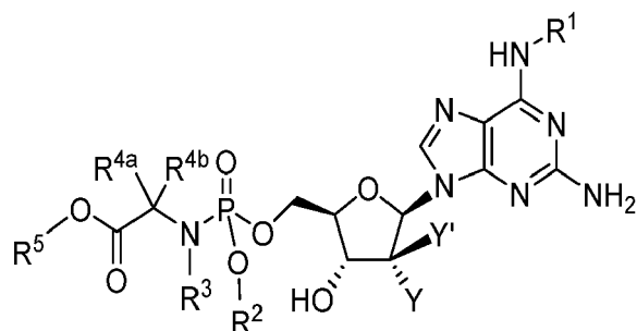
Formula V
