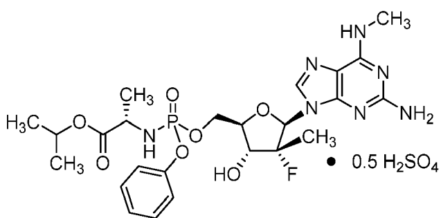
Compound 2
