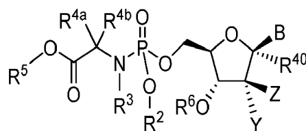
Formula VII
