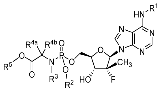
Formula II
