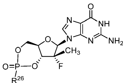
Formula VIII'
