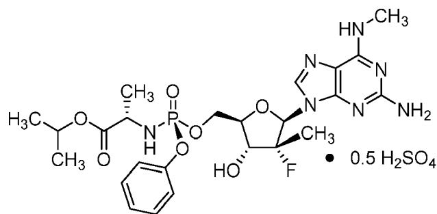
Compound 2A
