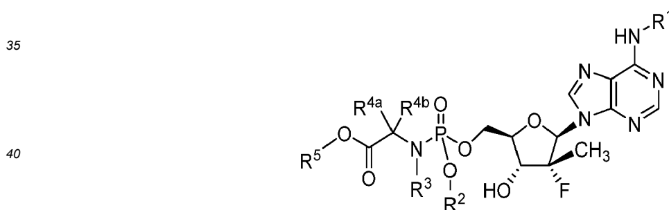
45 Formula II
