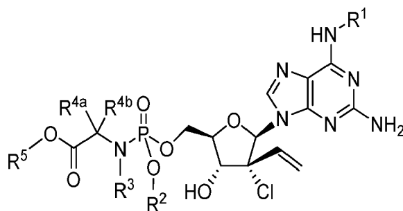
Formula IVd
