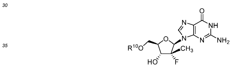
Formula VIII
