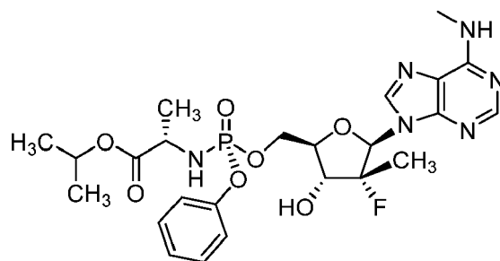
Compound 3B
