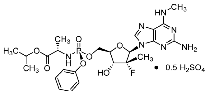
Compound 2A
