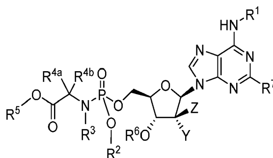
Formula VI
