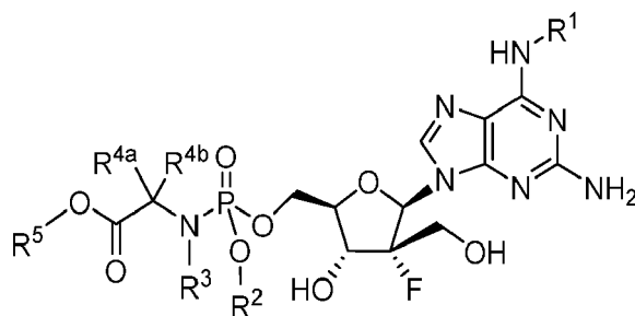
Formula IIIf
