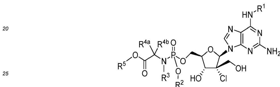
Formula IVf
