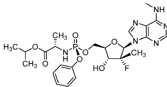
Compound 3A
