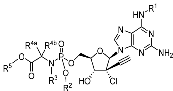
Formula IVe
