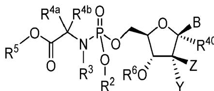
Formula VII
