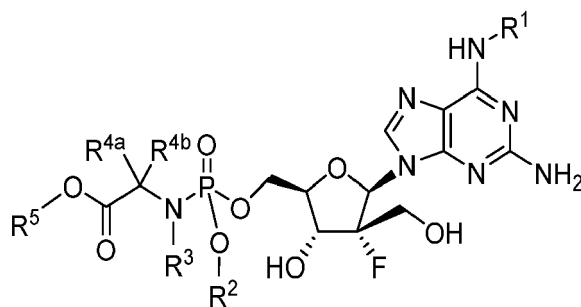
Formula IIIf
