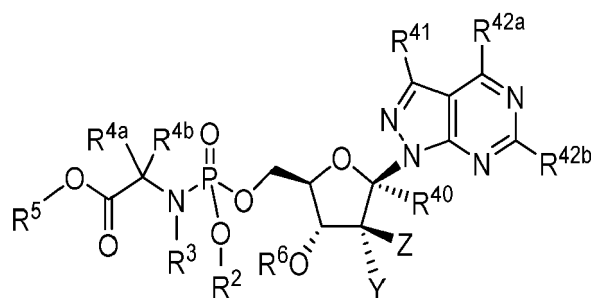
Formula VIIc
