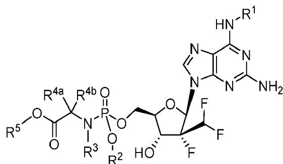
Formula IIIc
