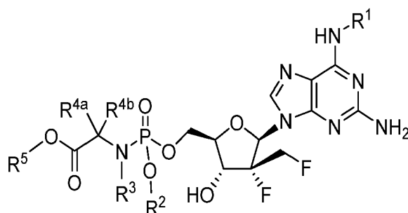
Formula IIIa
