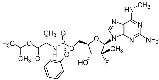
Compound 1B
