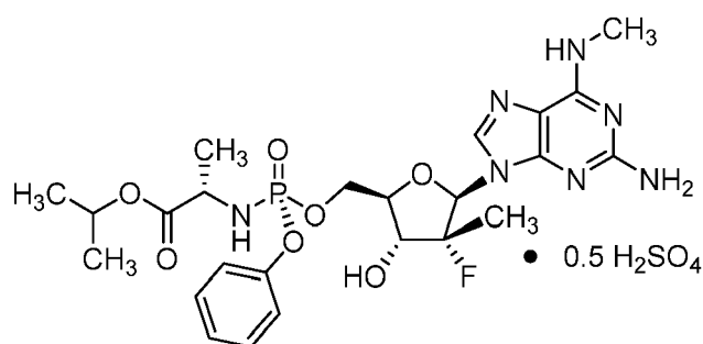
Compound 2B
