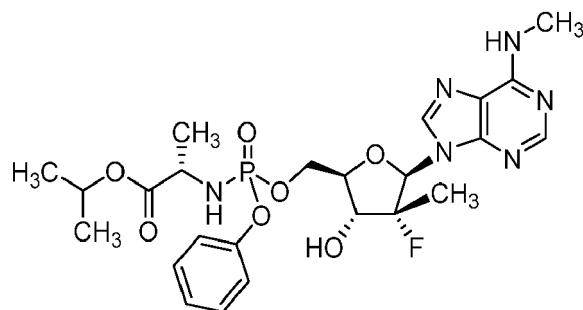
Compound 3
