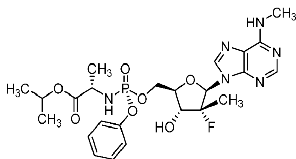
Compound 3B
