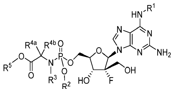
Formula IIIf
