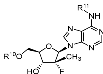
20 Formula X
