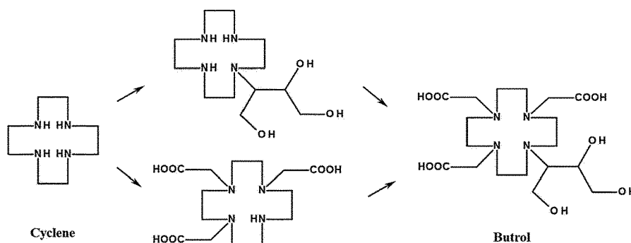
[Chemical Formula 5]
