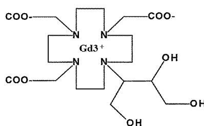
[Chemical Formula 4]
