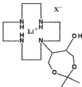
[Chemical Formula 1]
