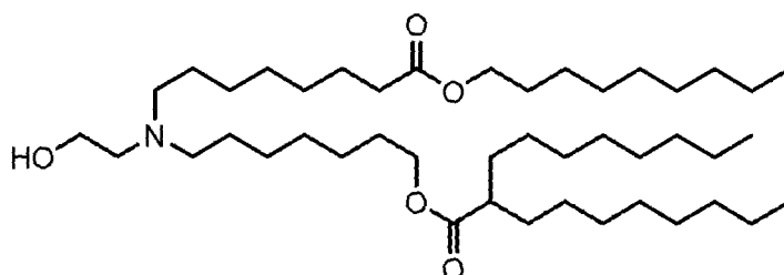
(Compound 30),
