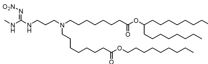
(Compound 200),
