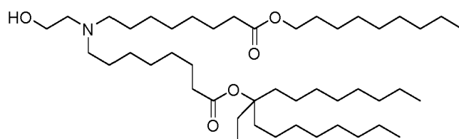
(Compound 83*),
