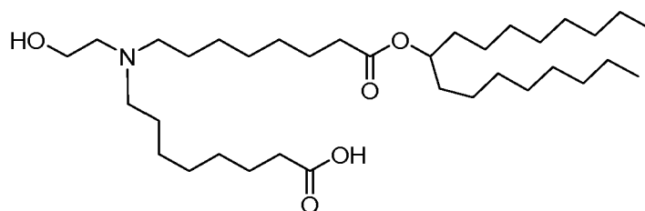
(Compound 166*),
