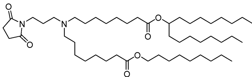
(Compound 176),
