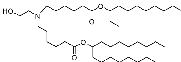
(Compound 91*),
