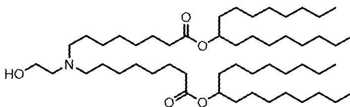
(Compound 29*),
