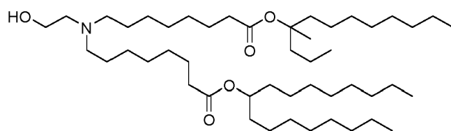
(Compound 87*),
