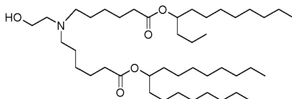
(Compound 92*),
