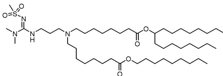
(Compound 213),
