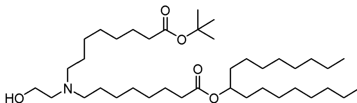
(Compound 155*),
