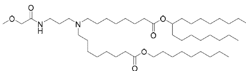
(Compound 178),
