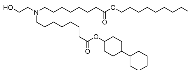
(Compound 80*),
