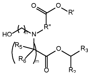
(IIc),
