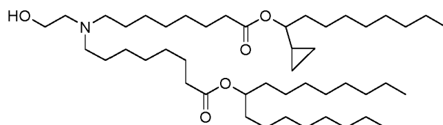
(Compound 65*),
