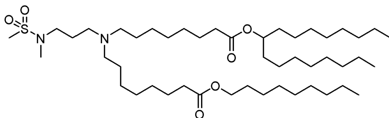
(Compound 173),
