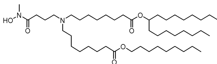
(Compound 227),
