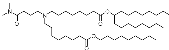
(Compound 224),
