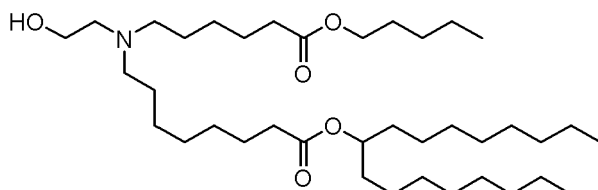
(Compound 104),
