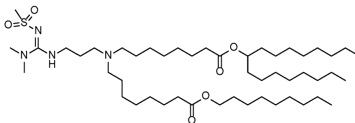
(Compound 213),
