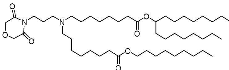
(Compound 202*),
