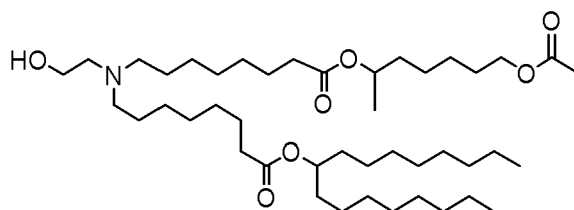
(Compound 214*),
