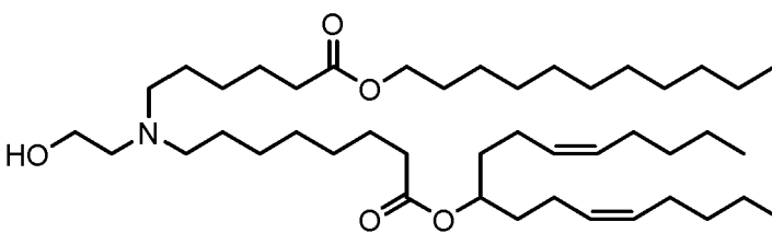
(Compound 61).
