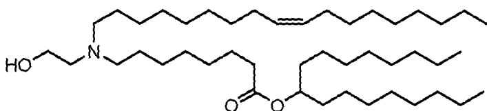
(Compound 31*),
