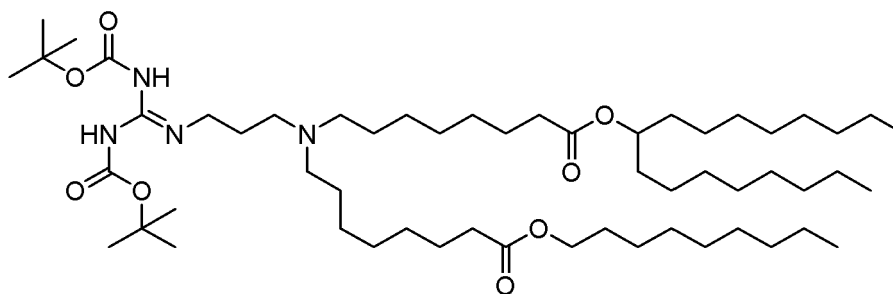
Chemical Formula: C_{56}H_{108}N_4O_8 Molecular Weight: 965.50
