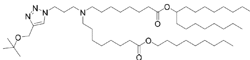
(Compound 177),
