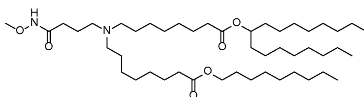
(Compound 226),
