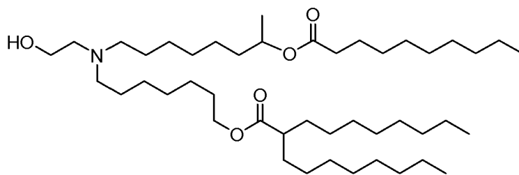
(Compound 165*),
