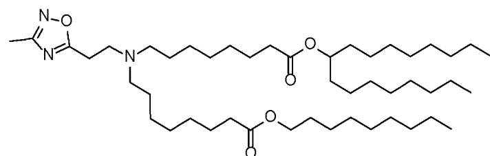
(Compound 230),
