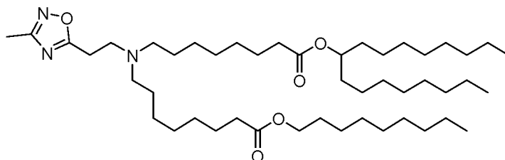
(Compound 230),
