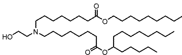
(Compound 33),
