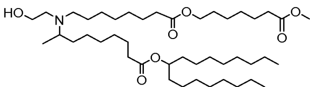
(Compound 192*),
