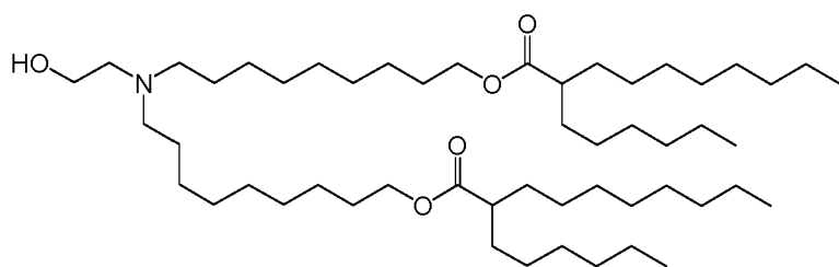
(Compound 133*),
