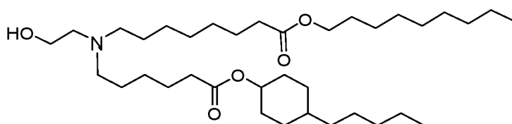
(Compound 232*),
