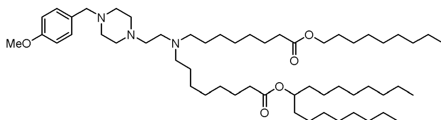
(Compound 102*),
