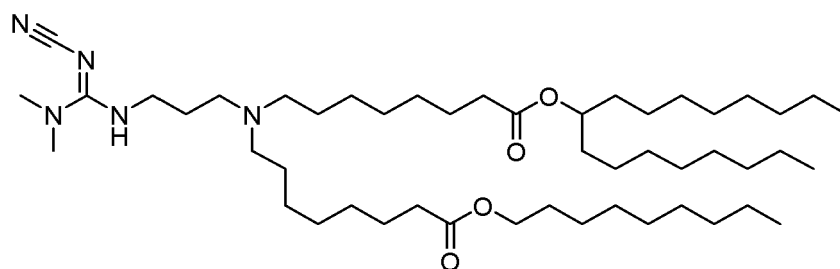
(Compound 168),
