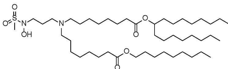
(Compound 206),
