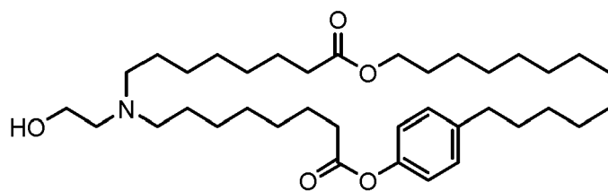
(Compound 64*).
