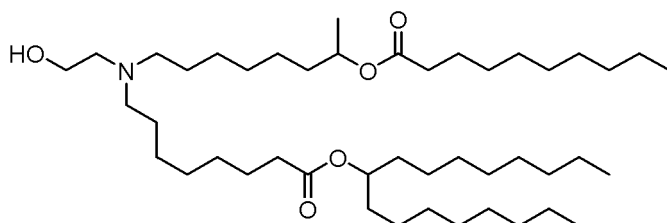
(Compound 98*),
