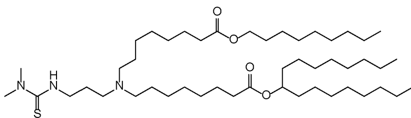
(Compound 111),
