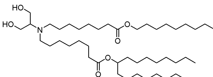
(Compound 156*),
