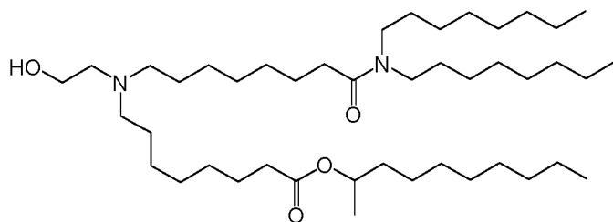
(Compound 130*),
