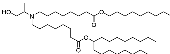
(Compound 157*),
