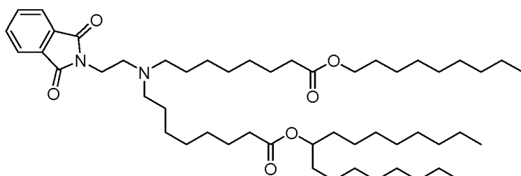
(Compound 100),
