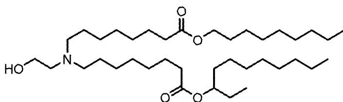
(Compound 35),
