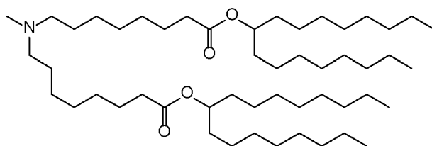
(Compound 124),
