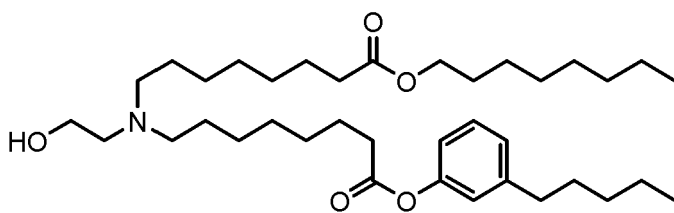
(Compound 63*),
