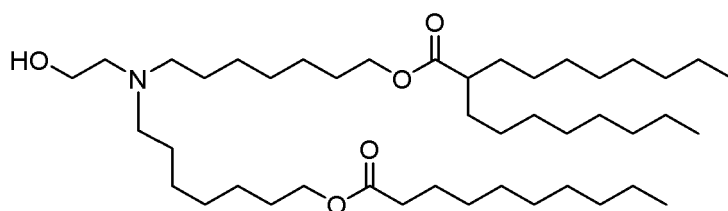
(Compound 151),
