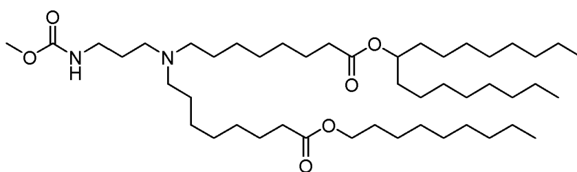
(Compound 181),
