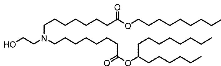
(Compound 32),
