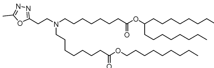
(Compound 231),
