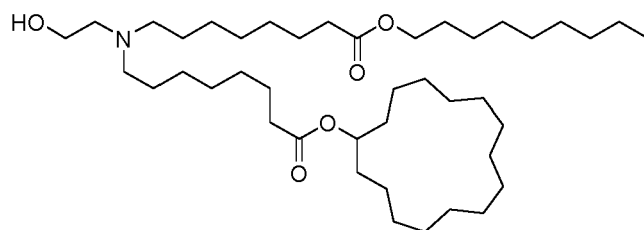
(Compound 81*),
