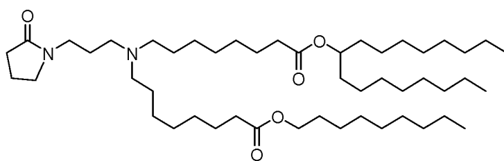
(Compound 195*),
