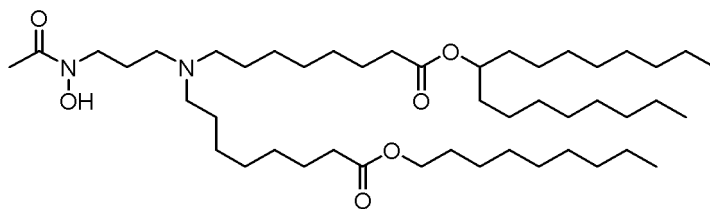
(Compound 204),
