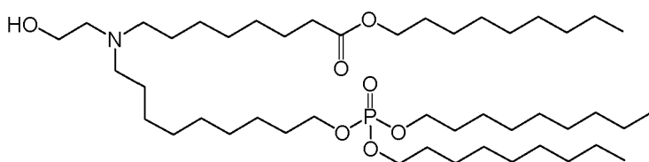
(Compound 127*),
