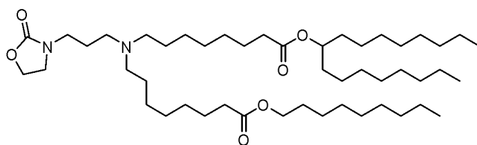
(Compound 199*),
