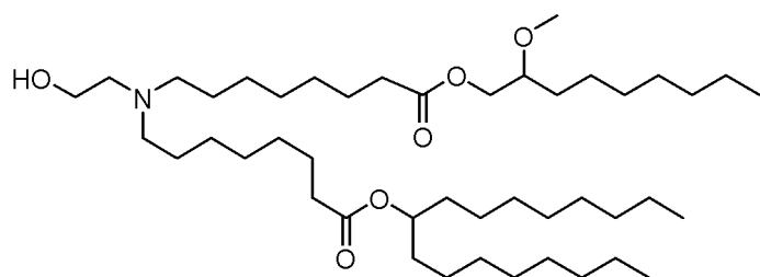
(Compound 148*),
