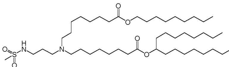
(Compound 109),
