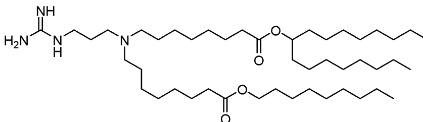
Chemical Formula: C_{46}H_{92}N_4O_4 Molecular Weight: 765.27
