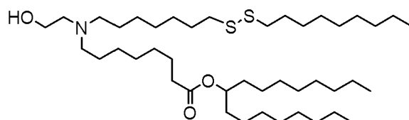
(Compound 215),
