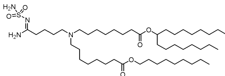
(Compound 221),
