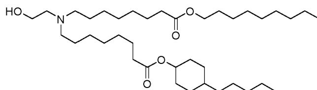
(Compound 79*),
