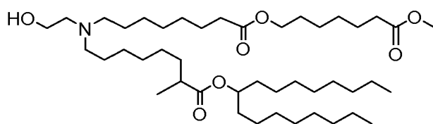
(Compound 190*),
