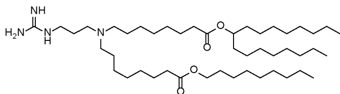
(Compound 207),
