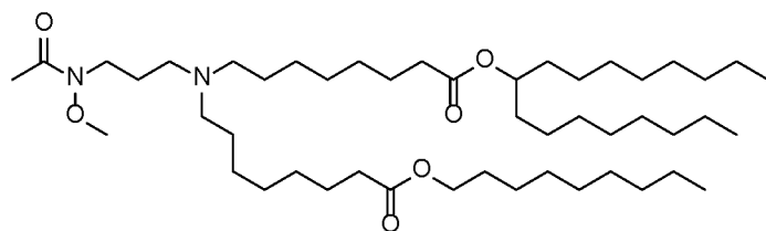
(Compound 203),
