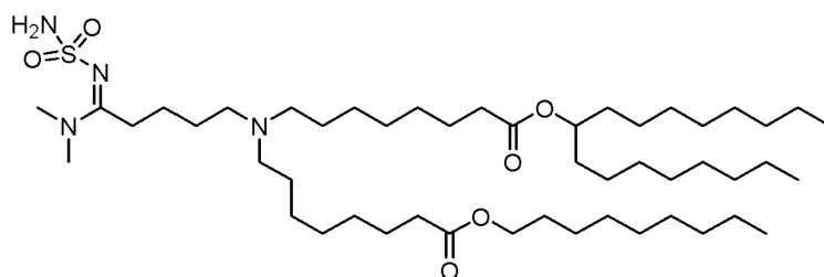
(Compound 219),
