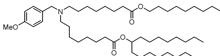
(Compound 95*),
