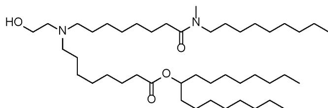
(Compound 105),
