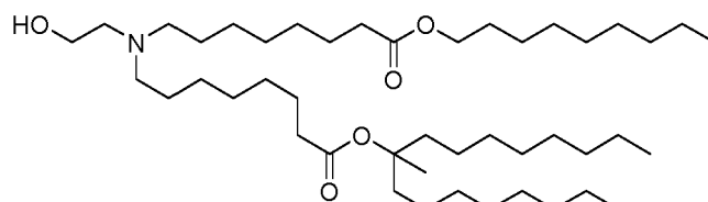
(Compound 82*),
