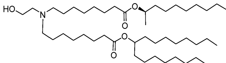
(Compound 172*),
