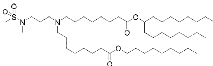
(Compound 173),
