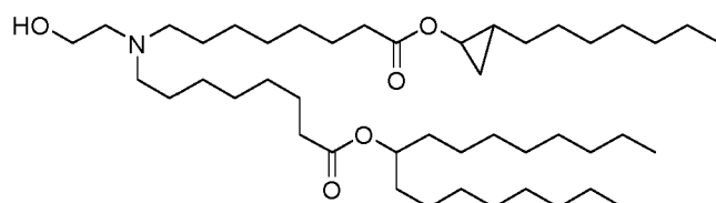
(Compound 93*),
