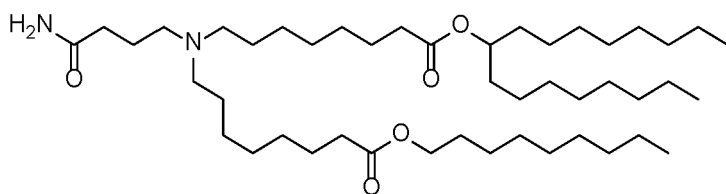
(Compound 222),
