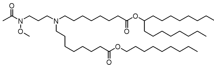
(Compound 203),
