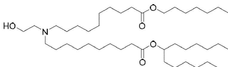
(Compound 186),
