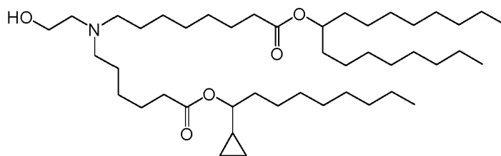
(Compound 128*),
