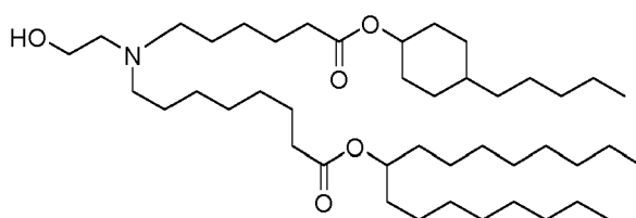
(Compound 68*),
