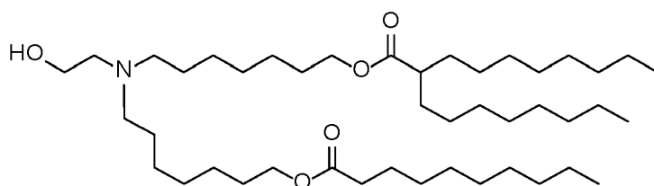
(Compound 151),
