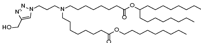
(Compound 218),
