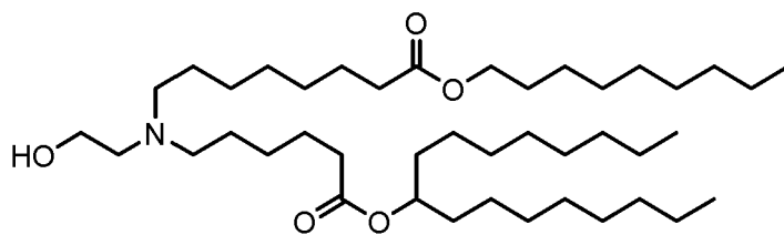
(Compound 27),
