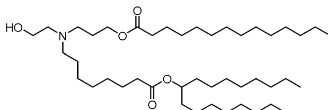
(Compound 97),
