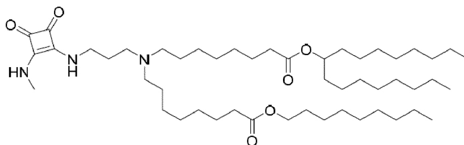
(Compound 182),
