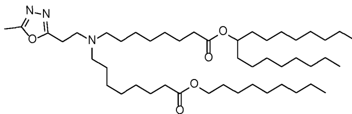
(Compound 231),
