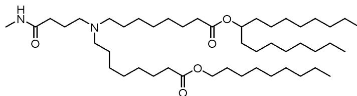
(Compound 223),
