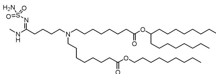
(Compound 220),
