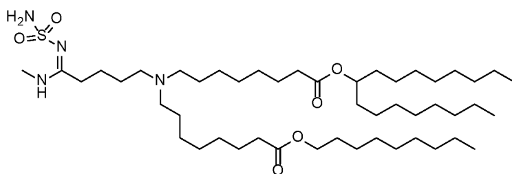
(Compound 220),
