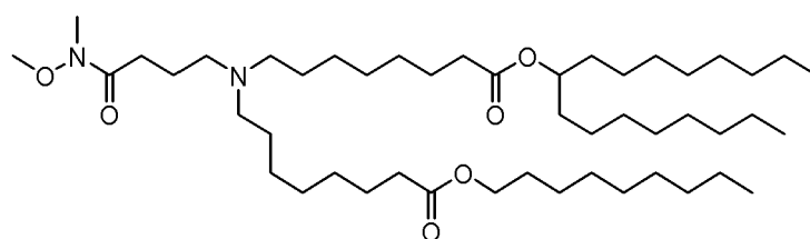
(Compound 228),
