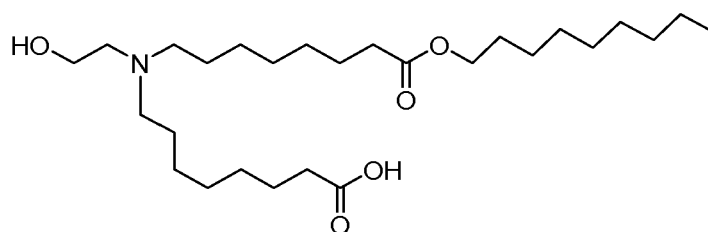
(Compound 167*),
