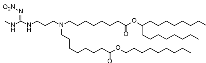
(Compound 200),
