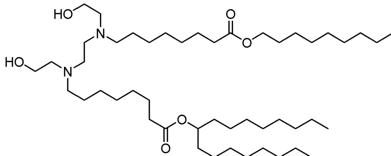
(Compound 159*),
