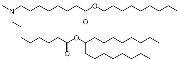
(Compound 123),
