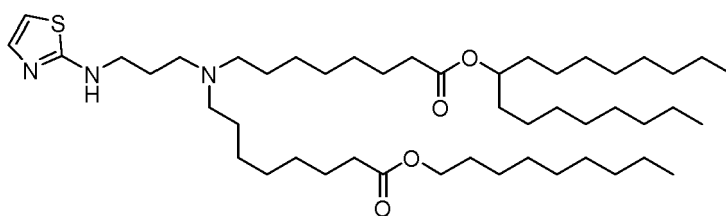
(Compound 208),
