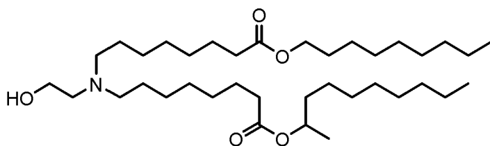
(Compound 36),
