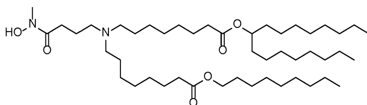
(Compound 227),
