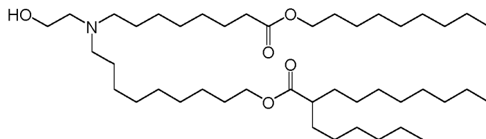
(Compound 134),
