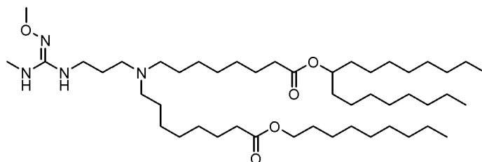
(Compound 210),
