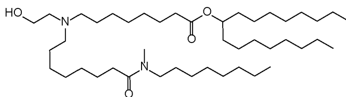
(Compound 145),
