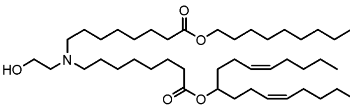
(Compound 60),
