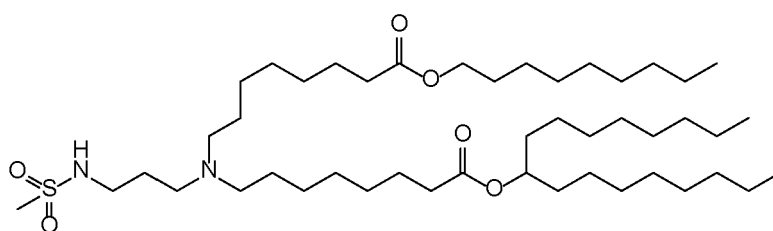
(Compound 109),
