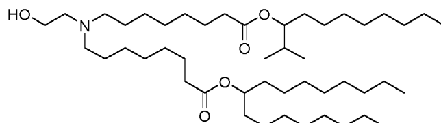
(Compound 78*),
