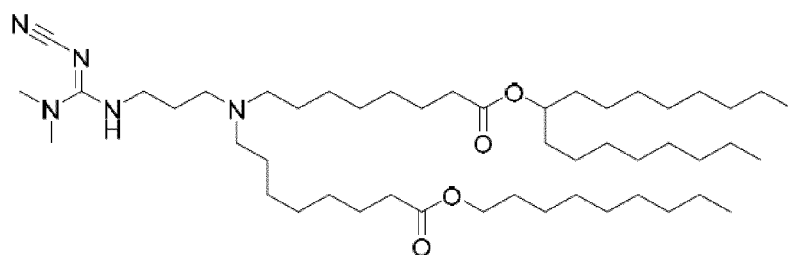
(Compound 168),
