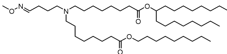
(Compound 229*),
