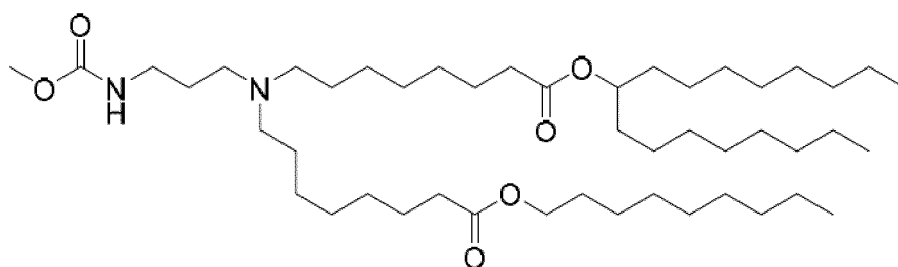
(Compound 181),
