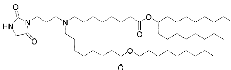
(Compound 174),
