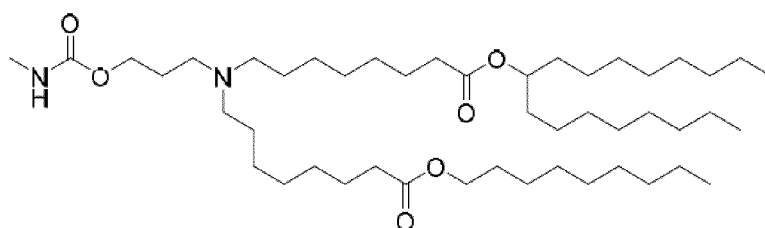
(Compound 175),
