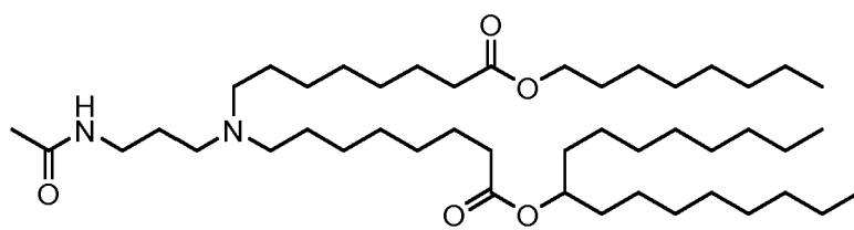
(Compound 37),
