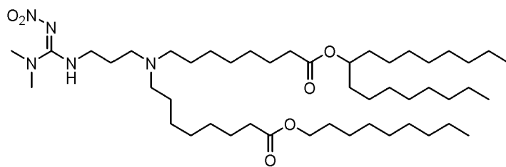
(Compound 209),
