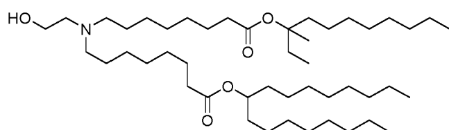
(Compound 86*),
