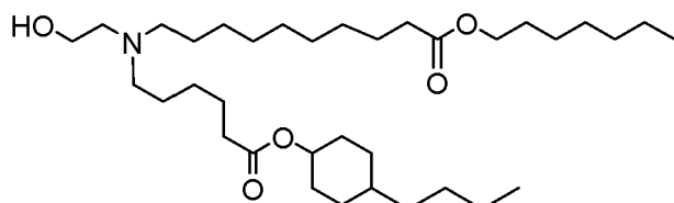
(Compound 191*),
