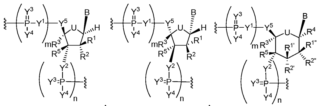
Formula IV
