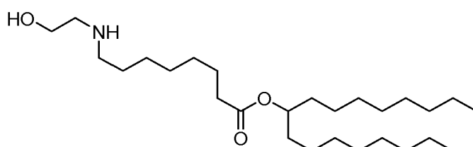
(Compound 180*),
