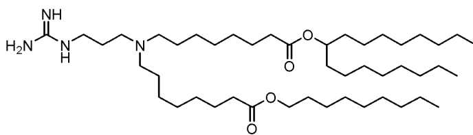
(Compound 207),
