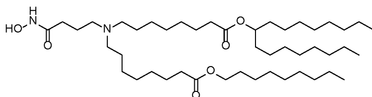
(Compound 225),
