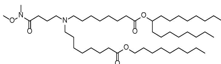
(Compound 228),
