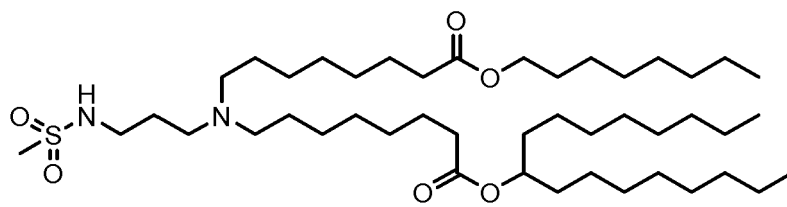
(Compound 38),
