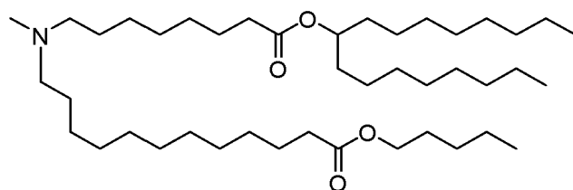
(Compound 150*),
