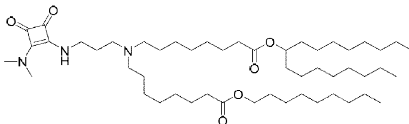
(Compound 169),
