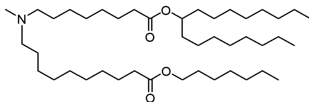
(Compound 149*),
