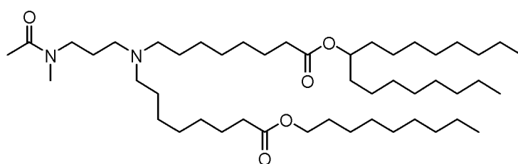
(Compound 196),
