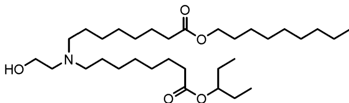
(Compound 59),
