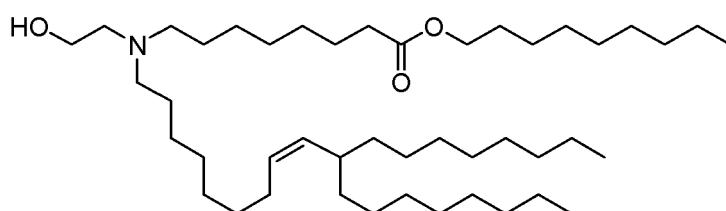
(Compound 152*),
