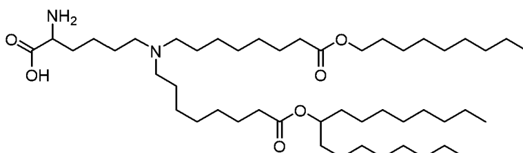
(Compound 106*),
