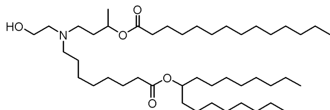
(Compound 99*),
