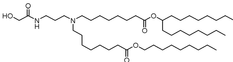
(Compound 198),
