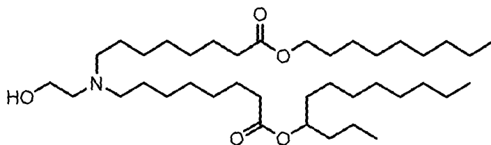
(Compound 34),
