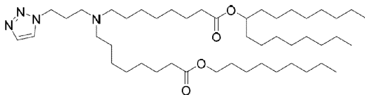
(Compound 179),
