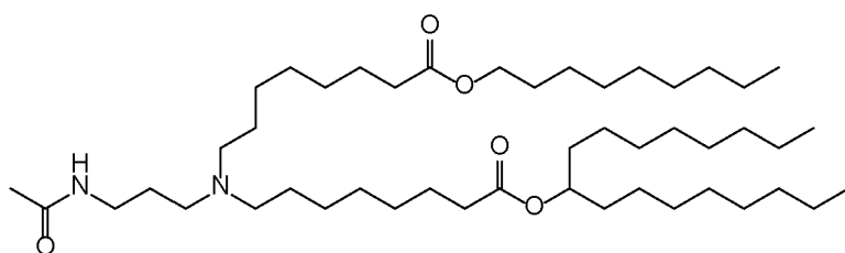
(Compound 108),
