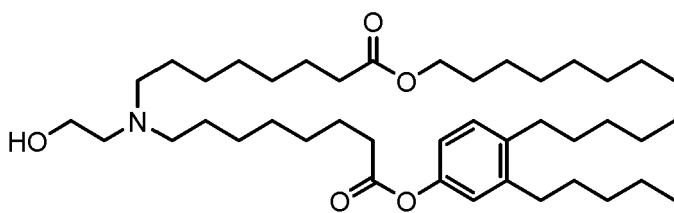
(Compound 62*),
