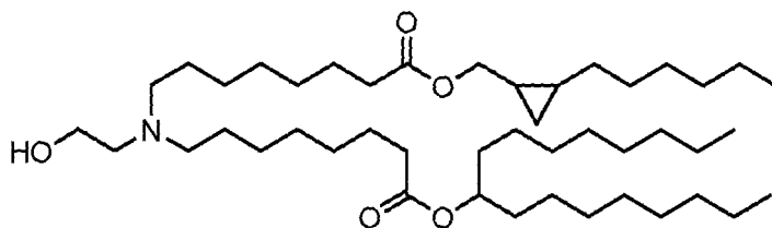
(Compound 28*),
