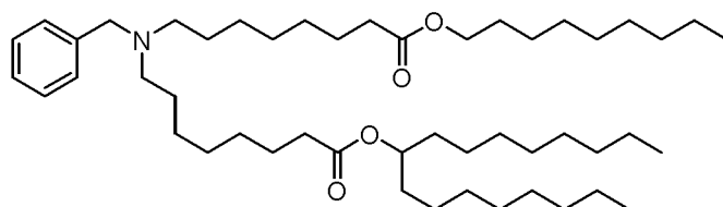
(Compound 94*),
