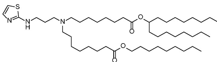
(Compound 208),
