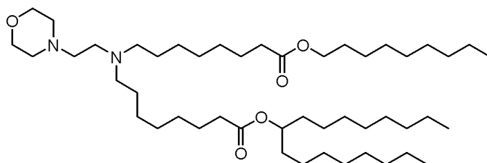
(Compound 103*),
