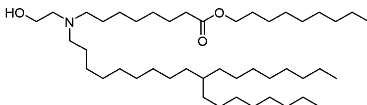
(Compound 153),
