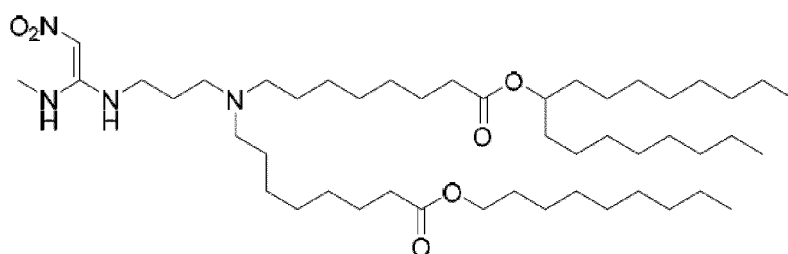
(Compound 170),
