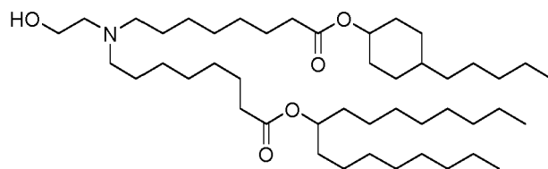
(Compound 66*),
