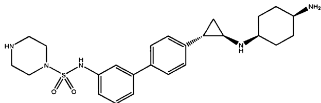
25 Example 104: N-(4'-((1R,2S)-2-((( trans )-4-aminocyclohexyl)amino)cyclopropyl)-[1,1'-biphenyl]-3-yl)piperazine-1-
