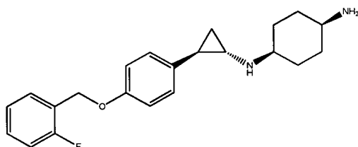
50 Example 106: ( trans )-N1-((1R,2S)-2-(4-((2-fluorobenzyl)oxy)phenyl)cyclopropyl)cyclohexane-1,4-diamine
