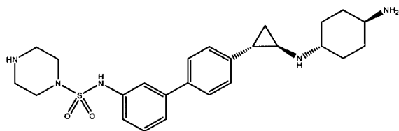
10 Example 103: N-(4'-((1S,2R)-2-((( cis )-4-aminocyclohexyl)amino)cyclopropyl)-[1,1'-biphenyl]-3-yl)piperazine-1-
