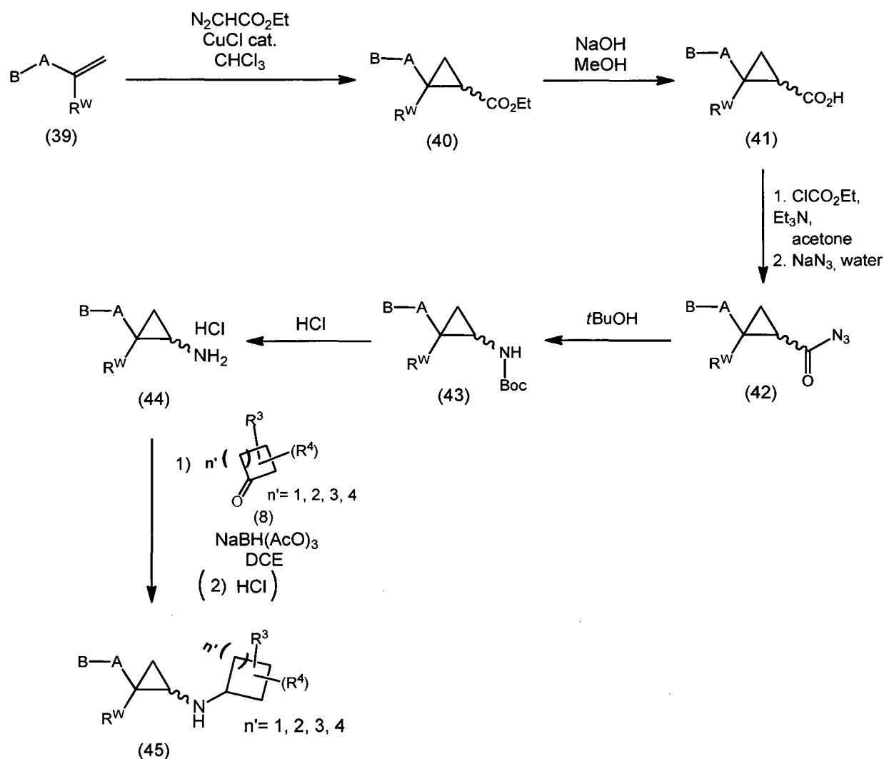
SCHEME 7: DCE (Dichloroethane)
